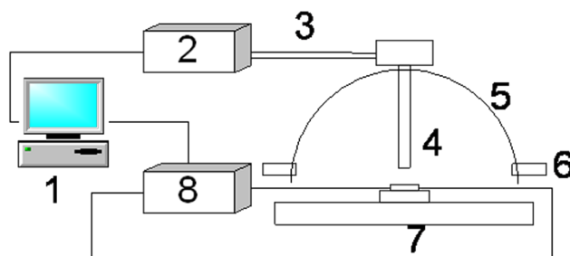
Fig. S1. System for measuring reflection spectra (1. Computer; 2. Spectrometer and Photoelectric converter; 3. Optical fiber; 4. Prober; 5. Integrating sphere; 6. Tungsten halogen lamp; 7. Sample stage; 8. DC power).
