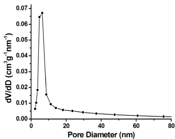
Fig. S2 BJH pore size distribution plots of mesoporous core-shell structure T3.
