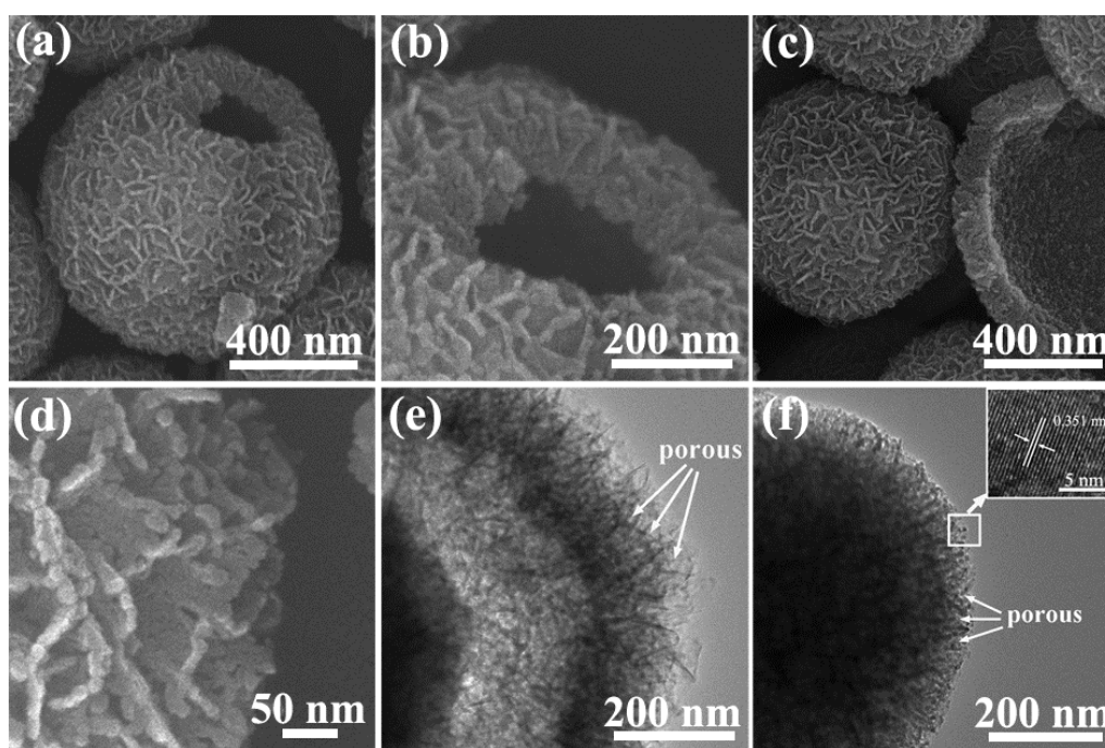
Fig. S1 (a-d) SEM images of the hierarchical TiO 2 core-shell spheres with different magnifications, (e) TEM image of as-prepared core-shell spheres, (f) TEM and HRTEM (inset) images of T2.
