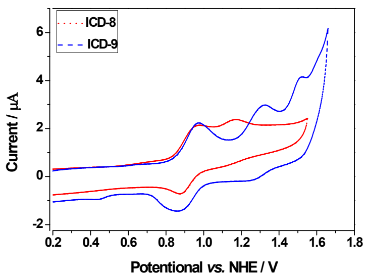
Fig.S2 The cyclic voltammograms of ICD-8 and ICD-9.
