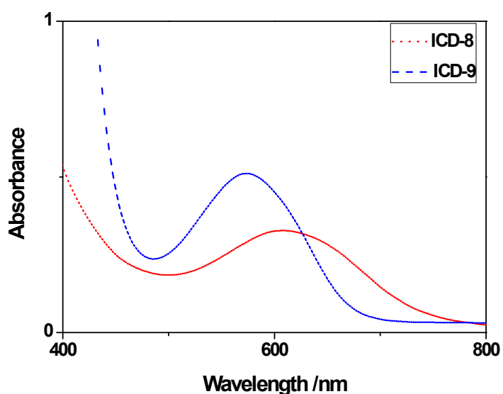
Fig.S1 The UV-Vis spectra of ICD-8 and ICD-9 on the TiO 2 .
