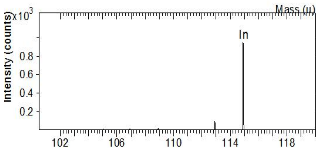
Figure S1. Mass spectra of In during SIMS sputtering
