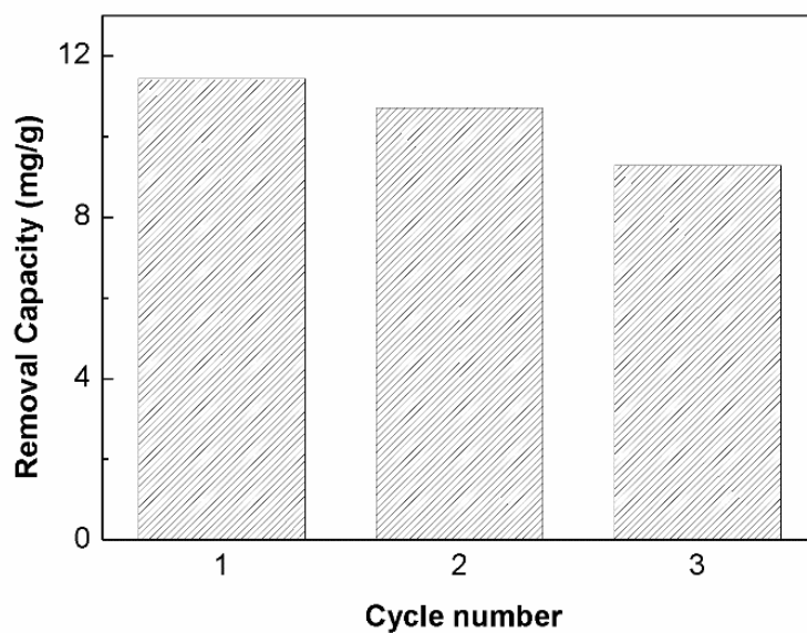
Fig. S1 Regeneration studies of \alpha\text{-Fe}_2\text{O}_3/\gamma\text{-Al}_2\text{O}_3 core/shell nanofibers after three cycles.
