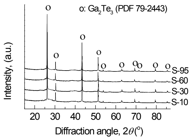
Supplementary Figure 1 XRD patterns of different samples.
