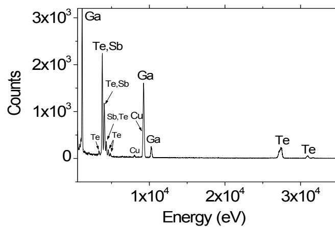
Supplementary Figure 2 The energy diffraction spectrum (EDS) of the alloy \text{Ga}_{1.9}\text{Cu}_{0.05}\text{Sb}_{0.1}\text{Te}_{2.95} .
