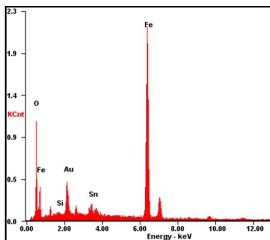
Fig. S1 EDS pattern of the Sn 4+ doped Fe 2 O 3 nanodiscs.
