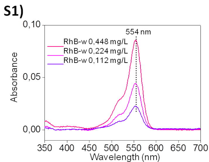
Figure S1 UV-VIS absorption spectra of RhB dissolved in water at different concentrations of dye (0,448; 0,224; 0,112 mg/L).
