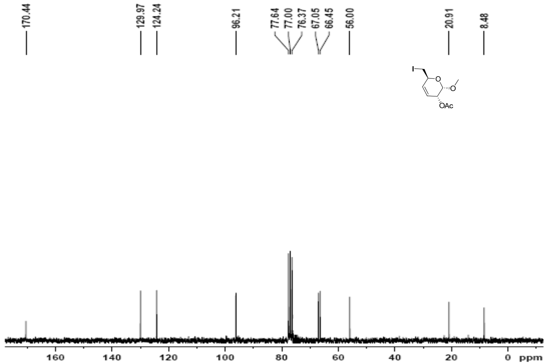
Figure 42 13 C NMR spectrum of compound 28
