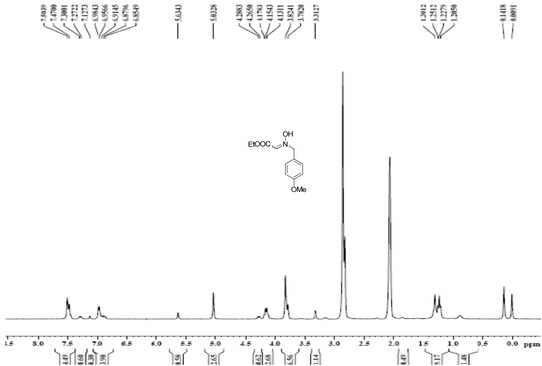
Figure 8 ^1\text{H} NMR spectrum of compound 5
