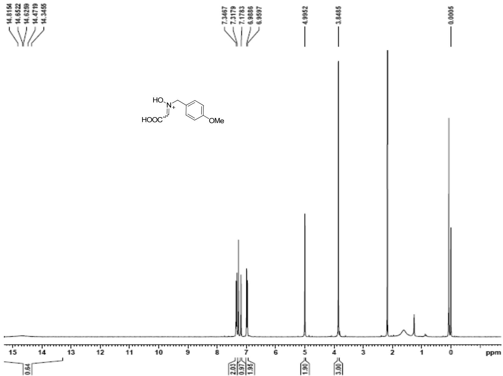
Figure 18 1 H NMR spectrum of compound 11
