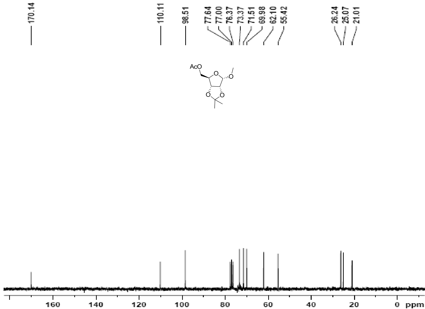
Figure 62 ^{13}\text{C} NMR spectrum of compound 39
