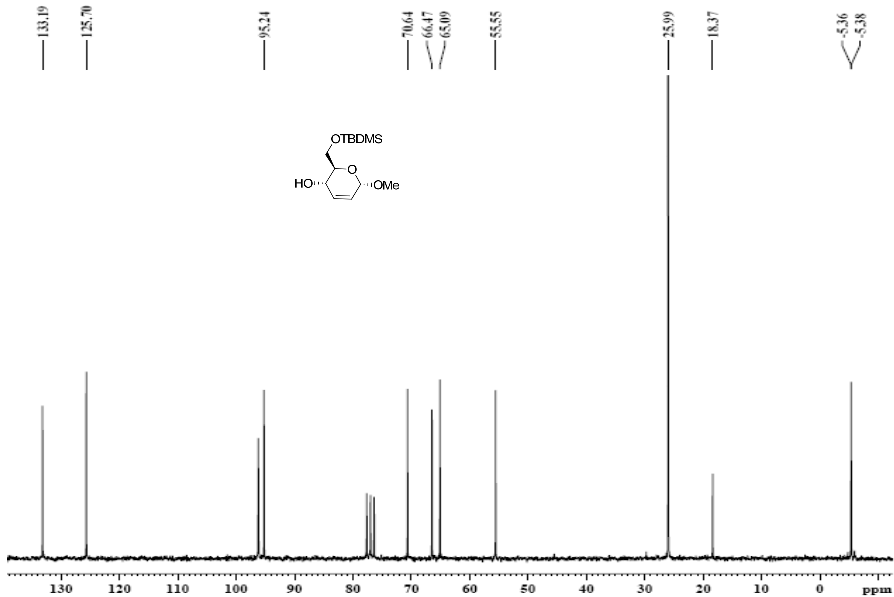
Figure 4 13 C NMR spectrum of compound 4
