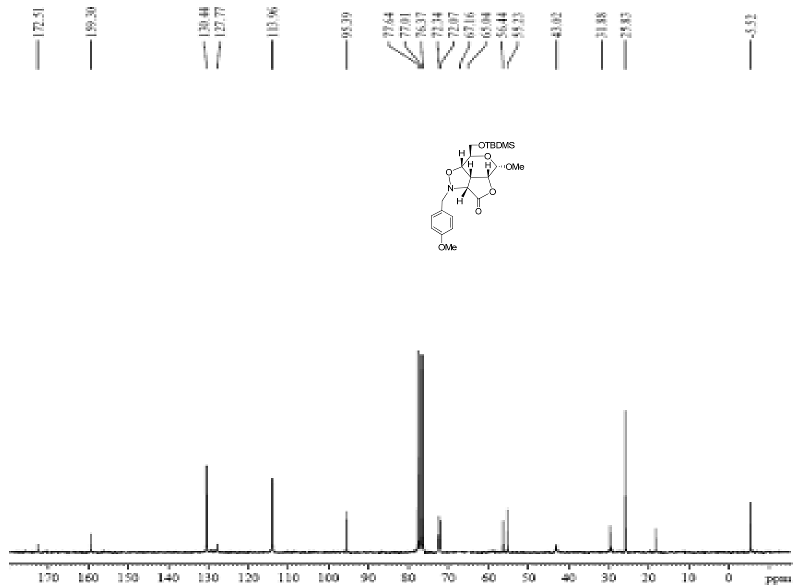
Figure 20 13 C NMR spectrum of compound 19
