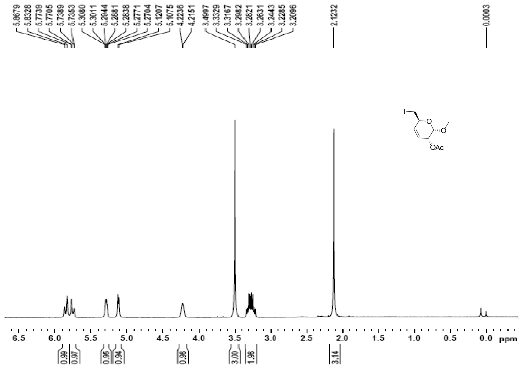
Figure 41 1 H NMR spectrum of compound 28
