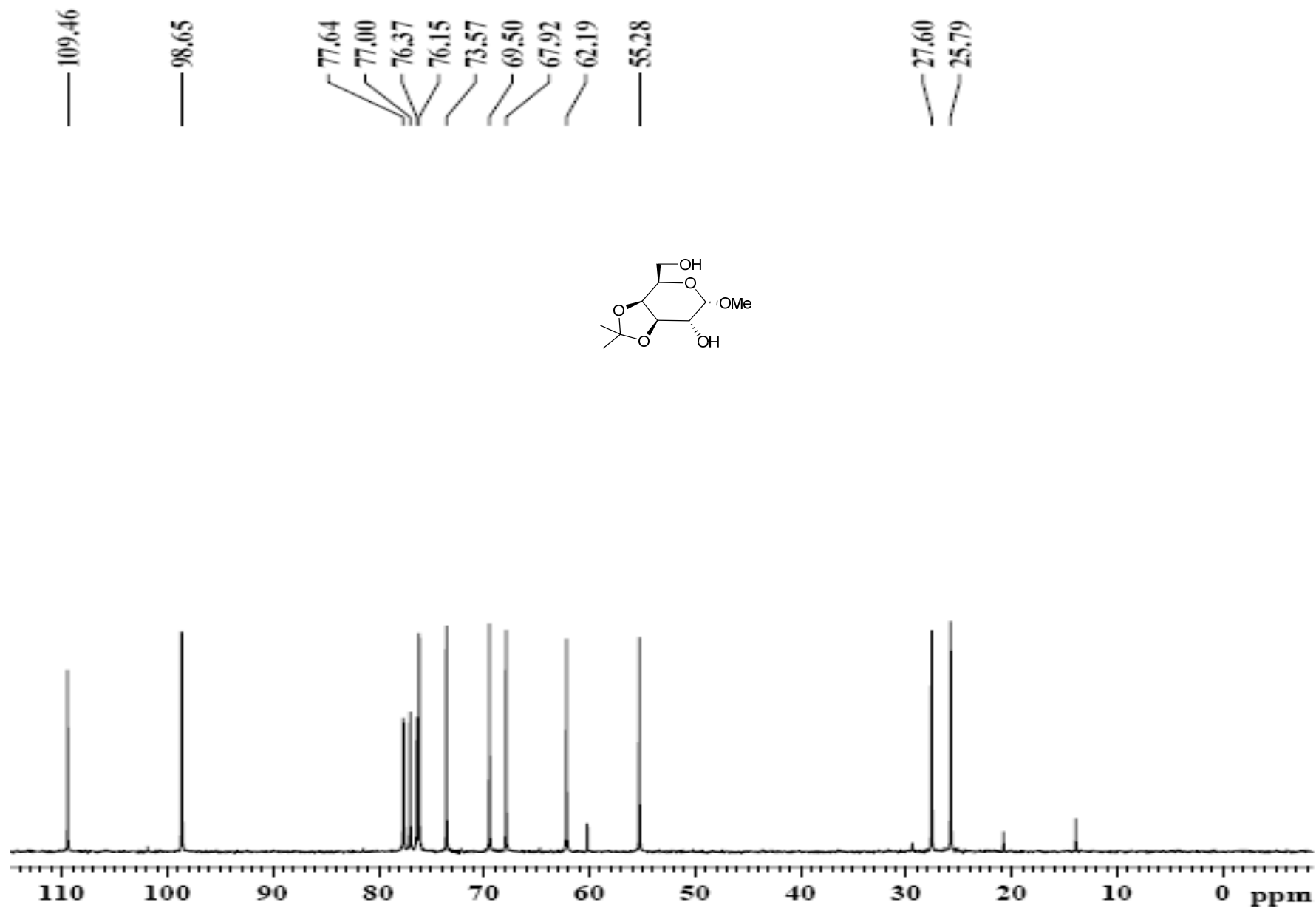
Figure 10 13 C NMR spectrum of compound 13
