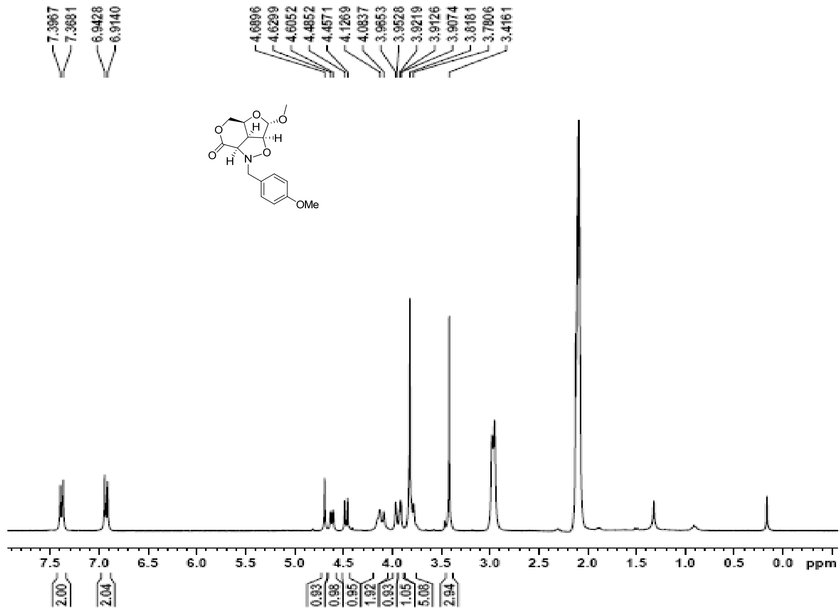
Figure 69 1 H NMR spectrum of compound 43
