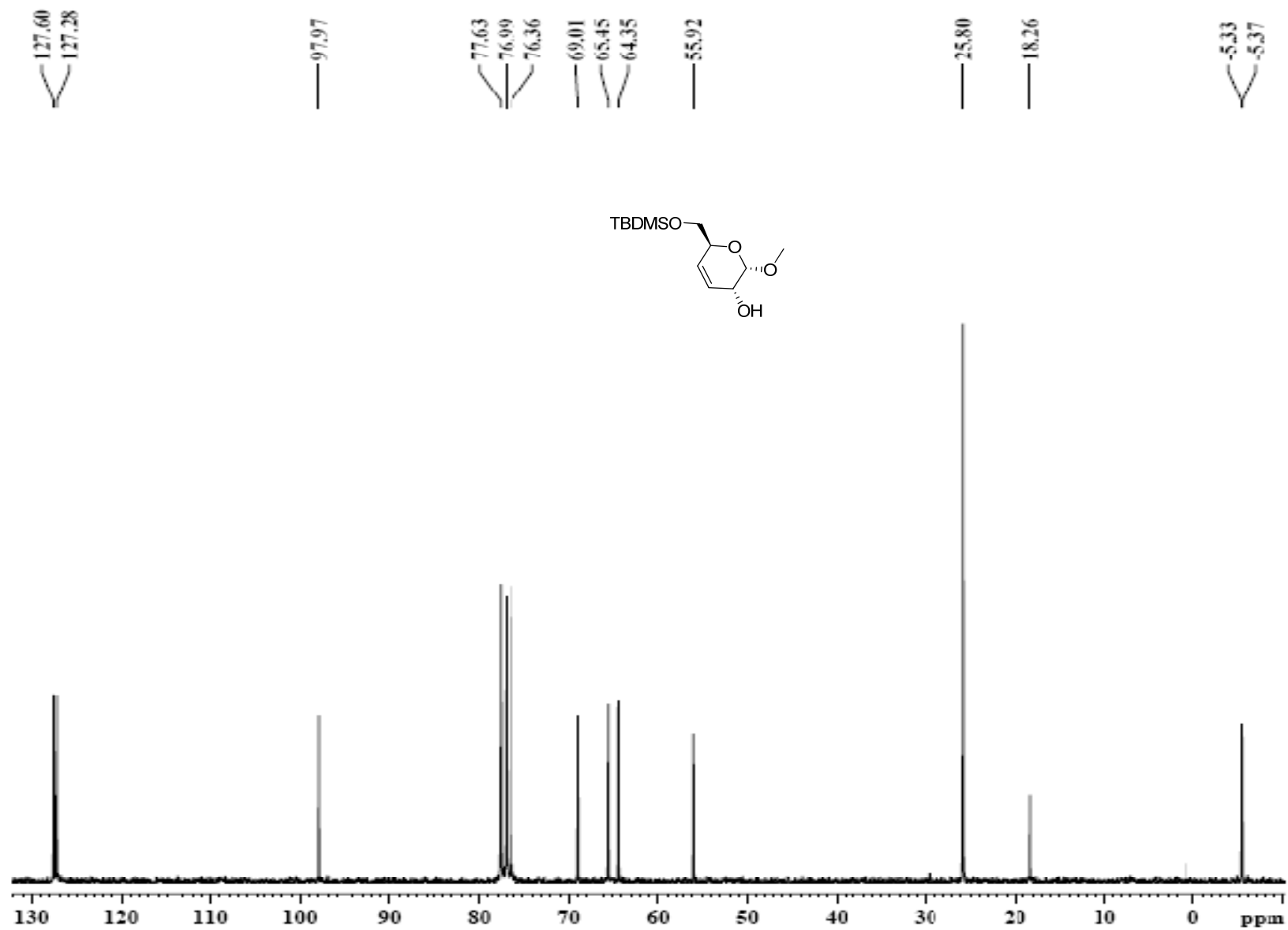
Figure 17 13 C NMR spectrum of compound 18
