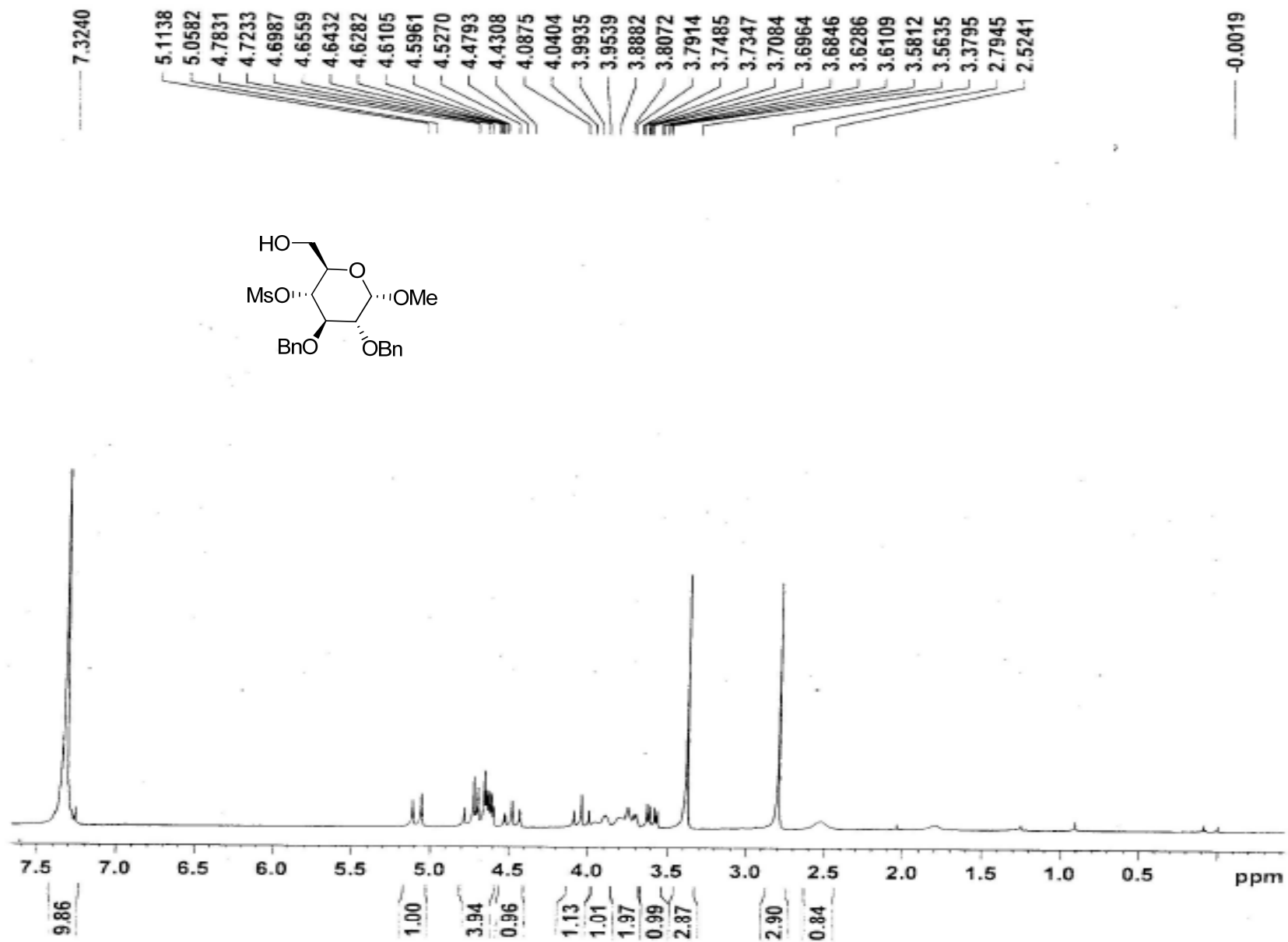
Figure 75 1 H NMR spectrum of compound 50
