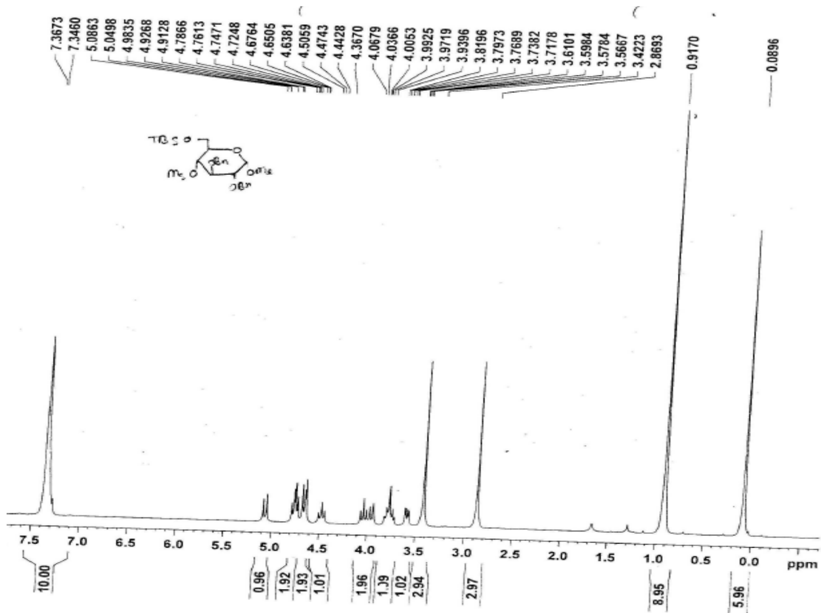
Figure 73 1 H NMR spectrum of compound 49
