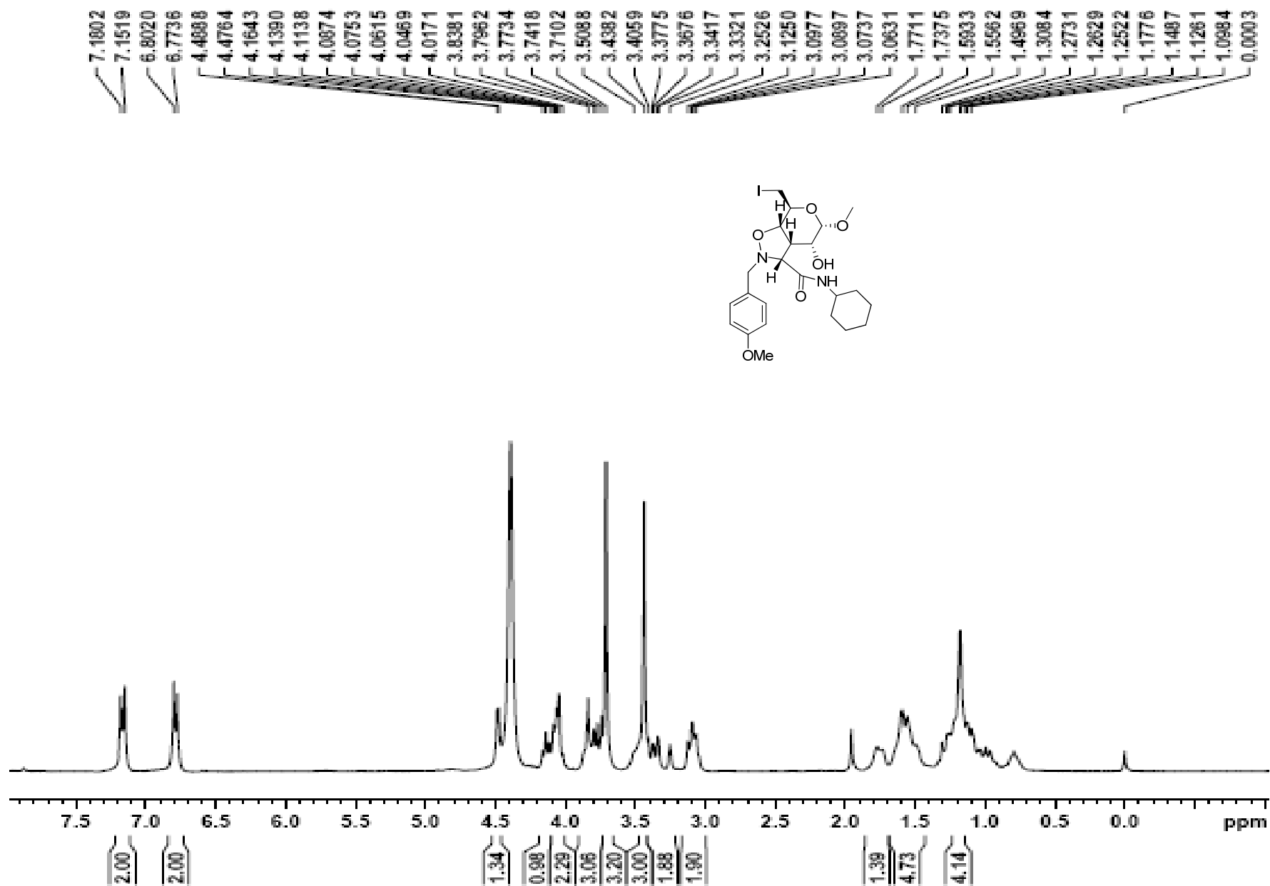
Figure 47 1 H NMR spectrum of compound 30b
