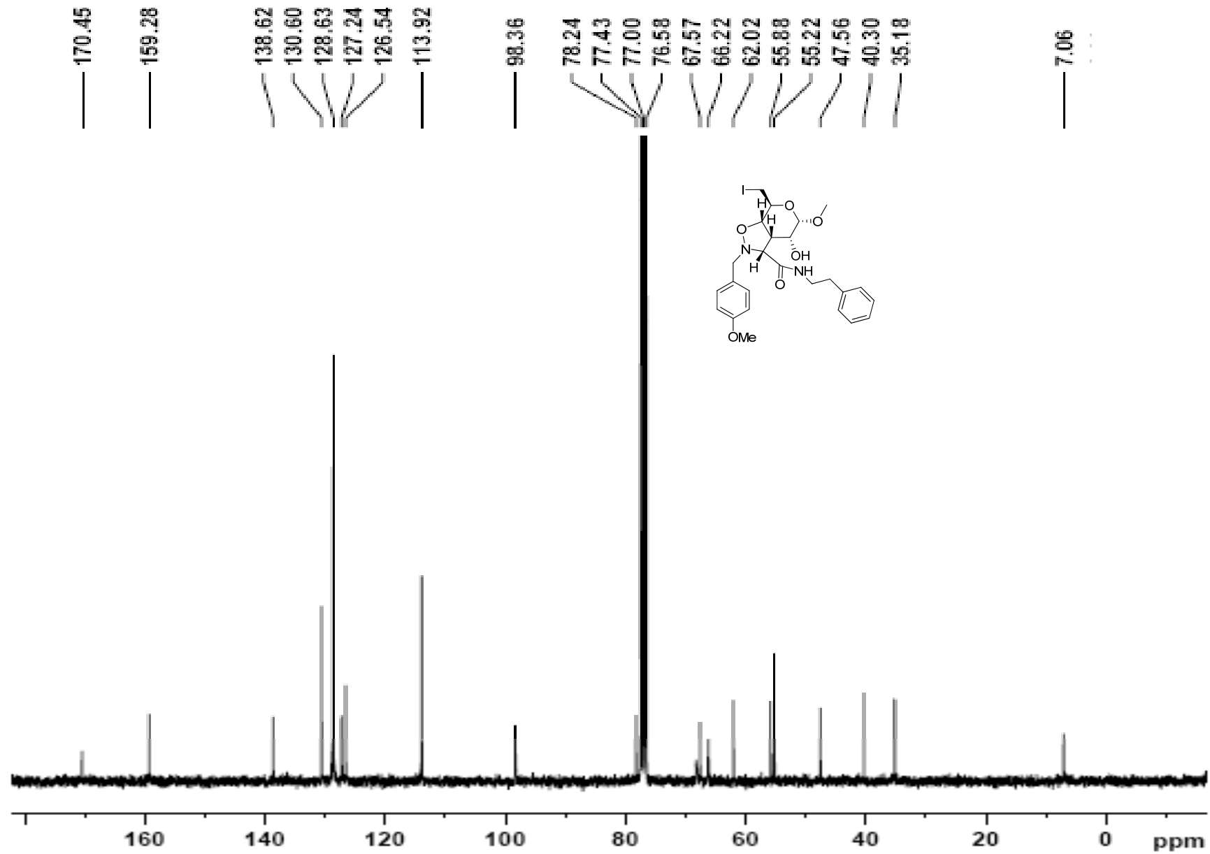
Figure 50 ^{13}\text{C} NMR spectrum of compound 30c
