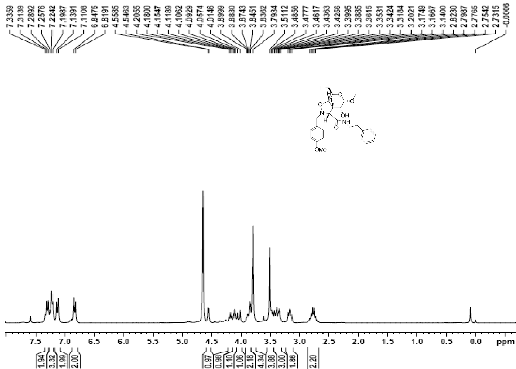
Figure 49 1 H NMR spectrum of compound 30c
