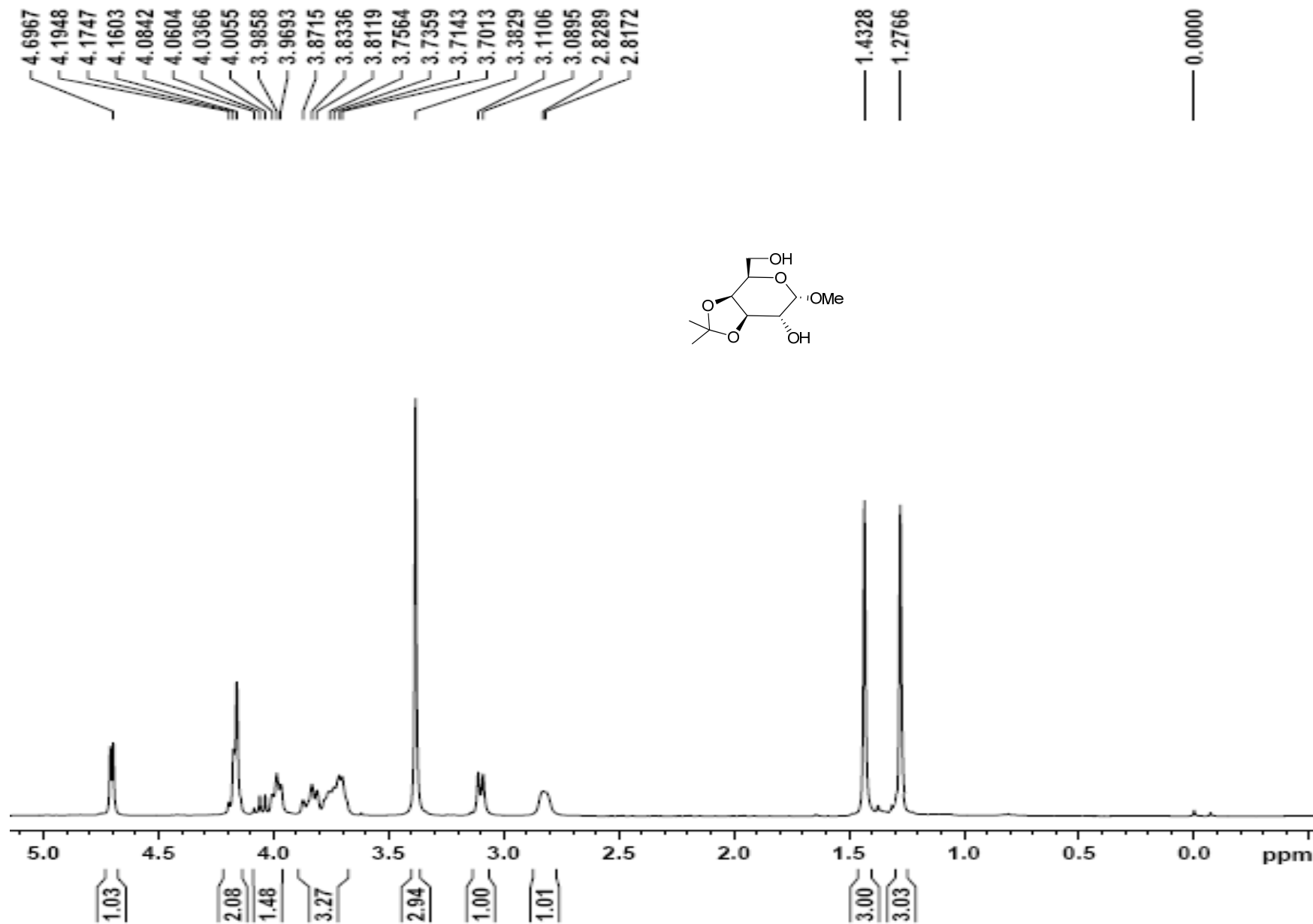
Figure 9 1 H NMR spectrum of compound 13
