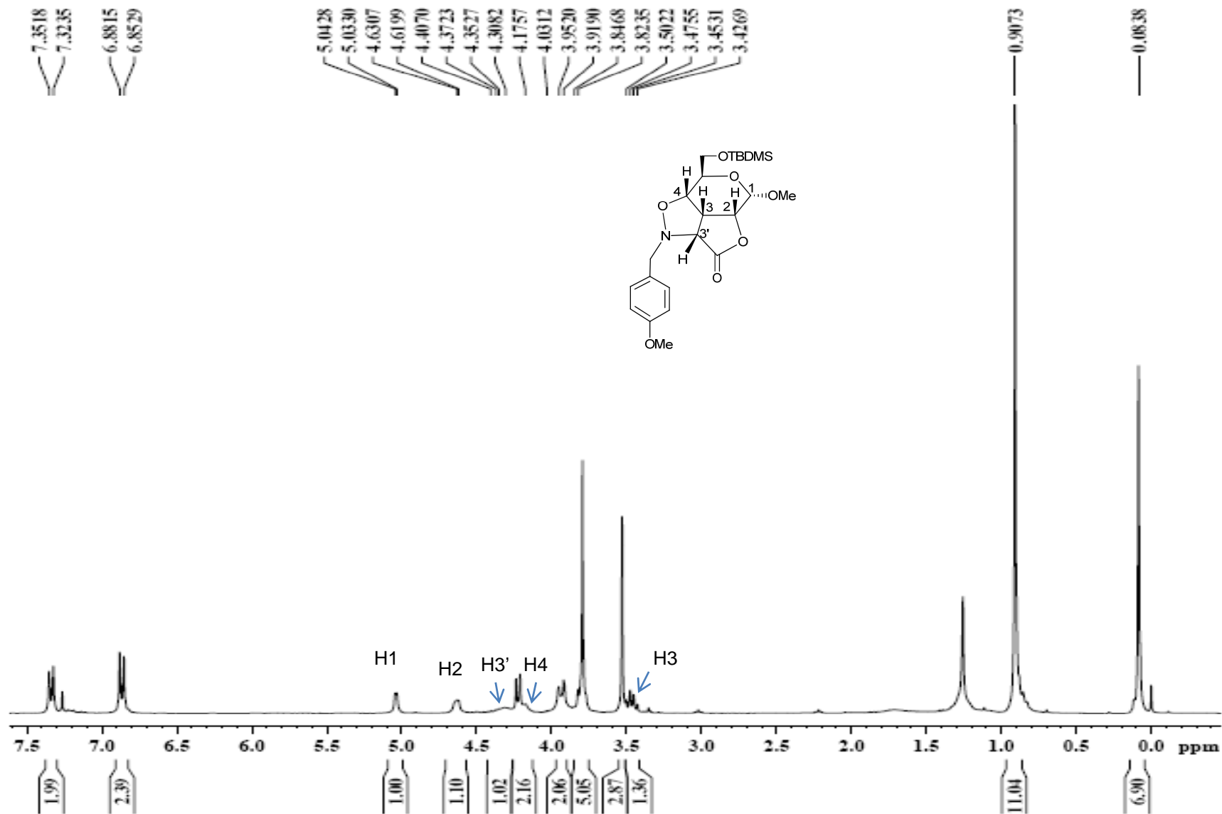
Figure 19 1 H NMR spectrum of compound 19
