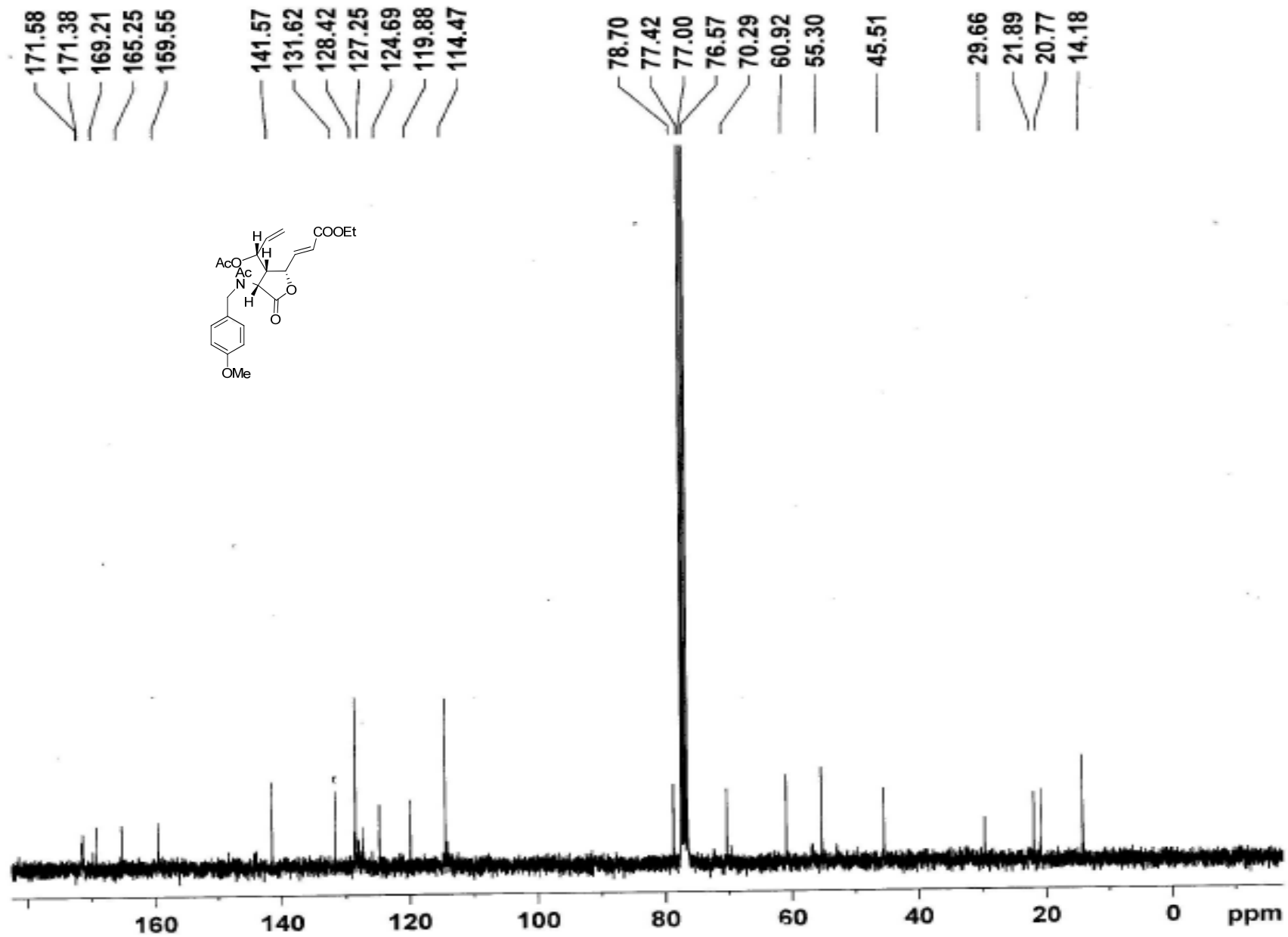
Figure 58 ^{13}\text{C} NMR spectrum of compound 36
