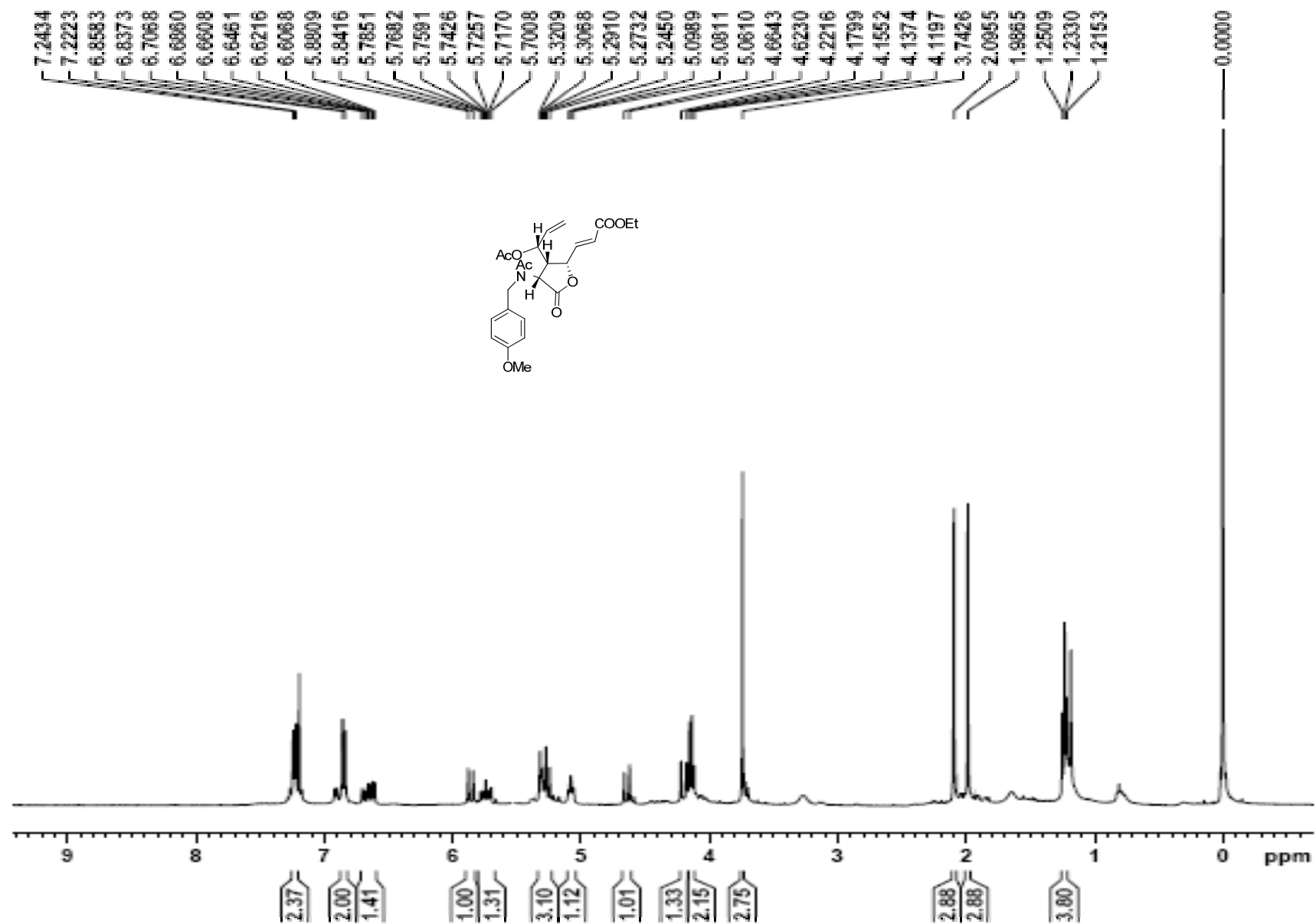
Figure 57 1 H NMR spectrum of compound 36
