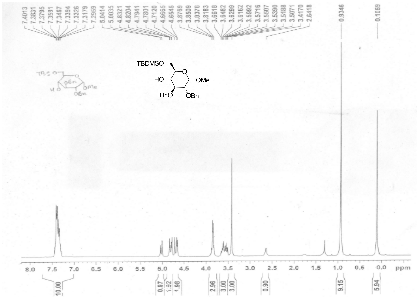
Figure 71 1 H NMR spectrum of compound 48
