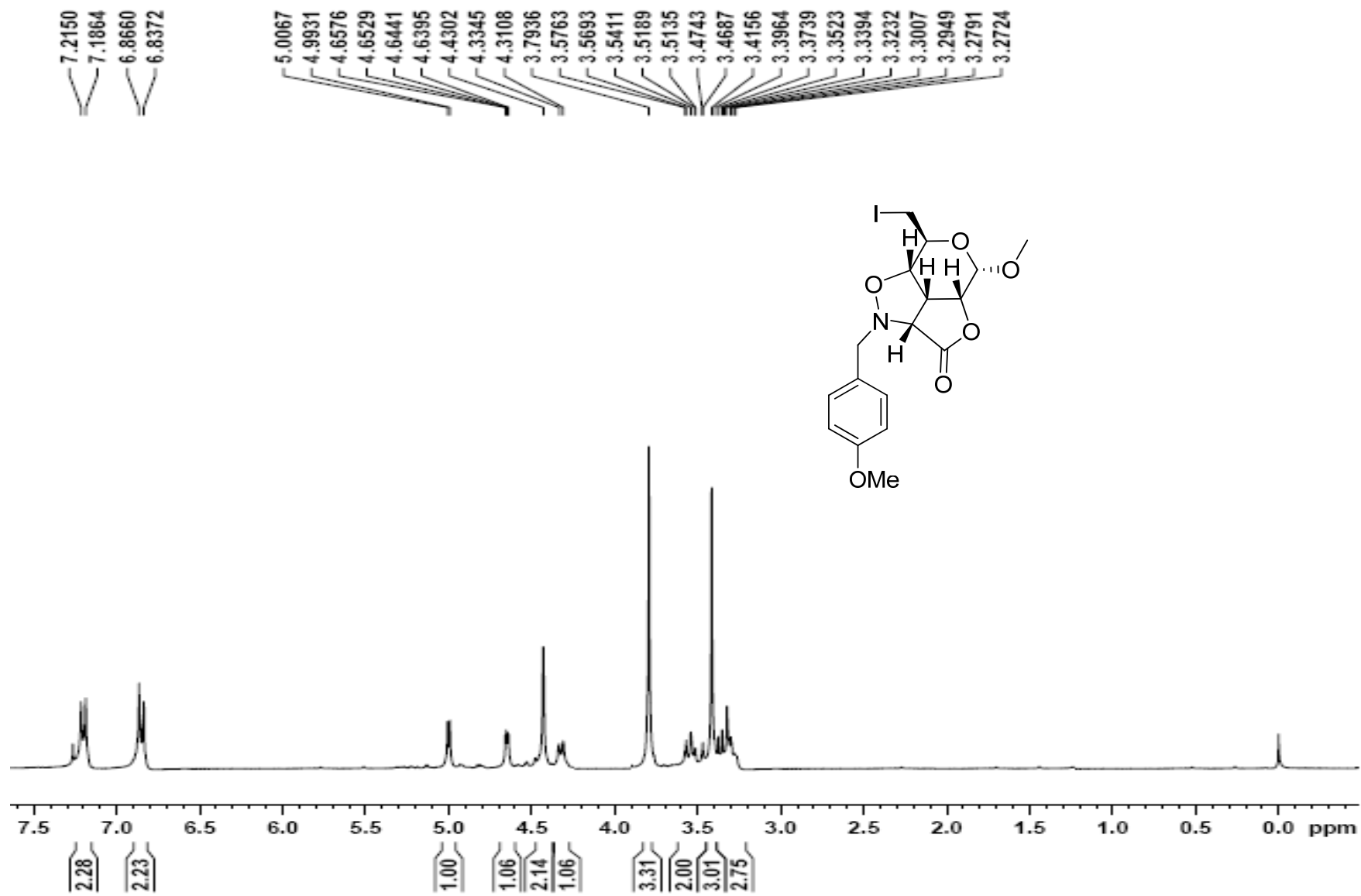
Figure 28 ^1\text{H} NMR spectrum of compound 21
