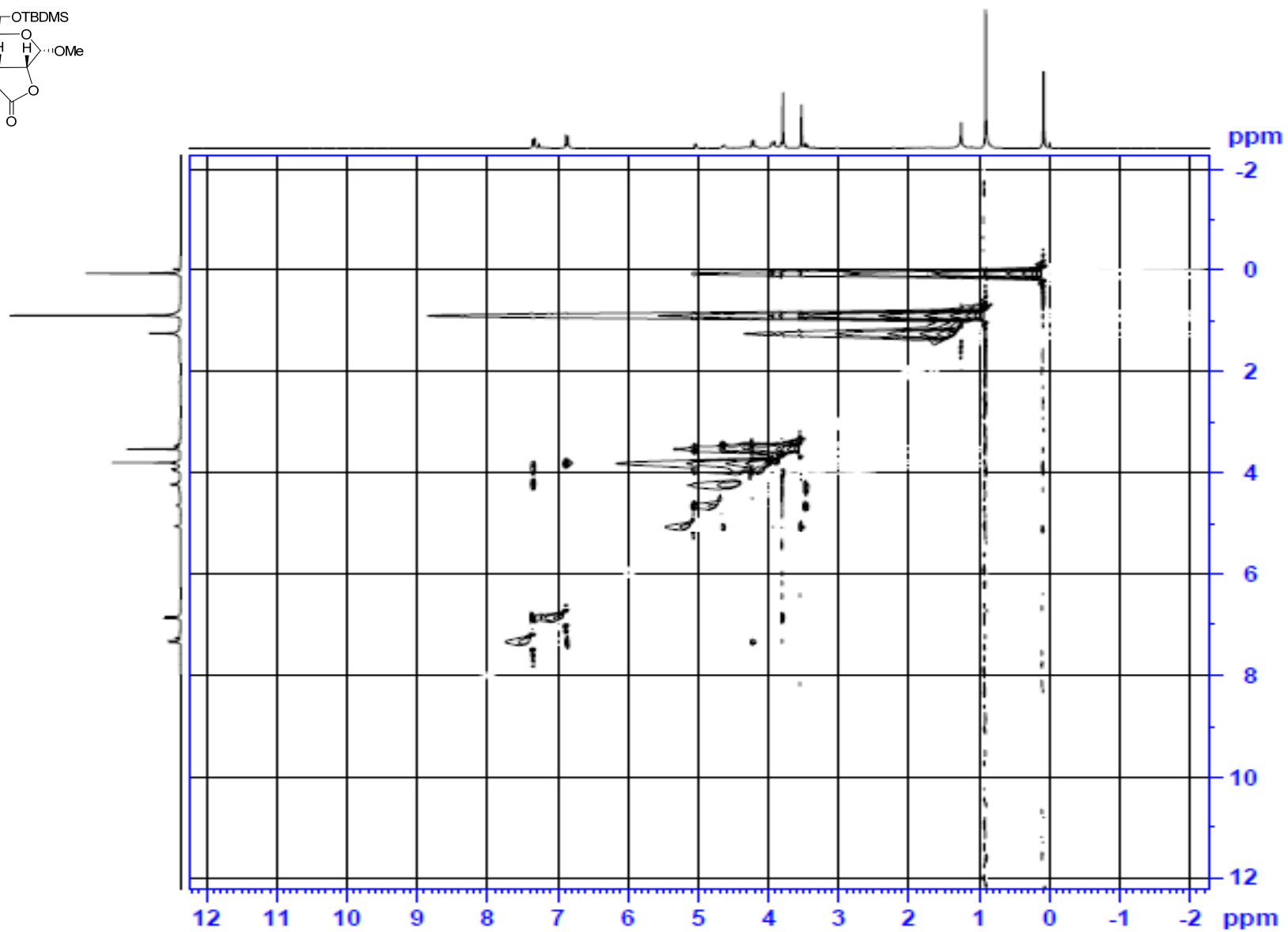
Figure 25 NOESY spectrum of compound 19
