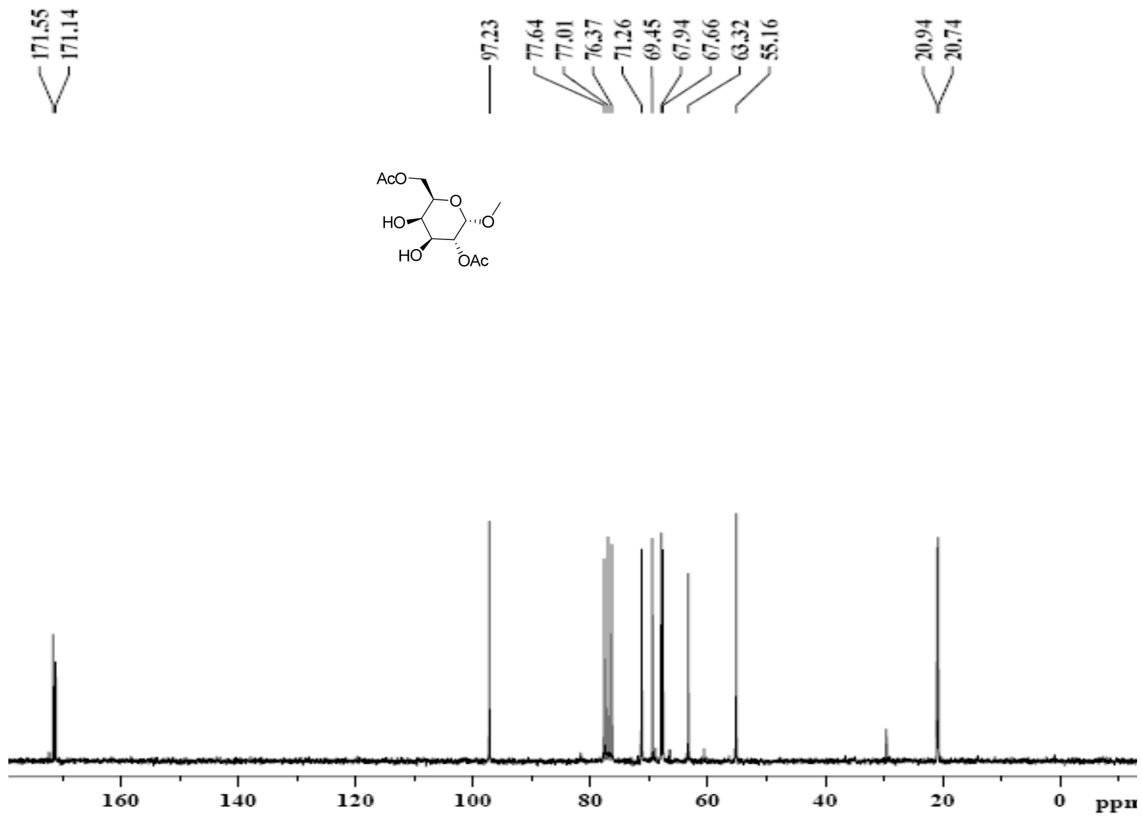
Figure 14 ^{13}\text{C} NMR spectrum of compound 15
