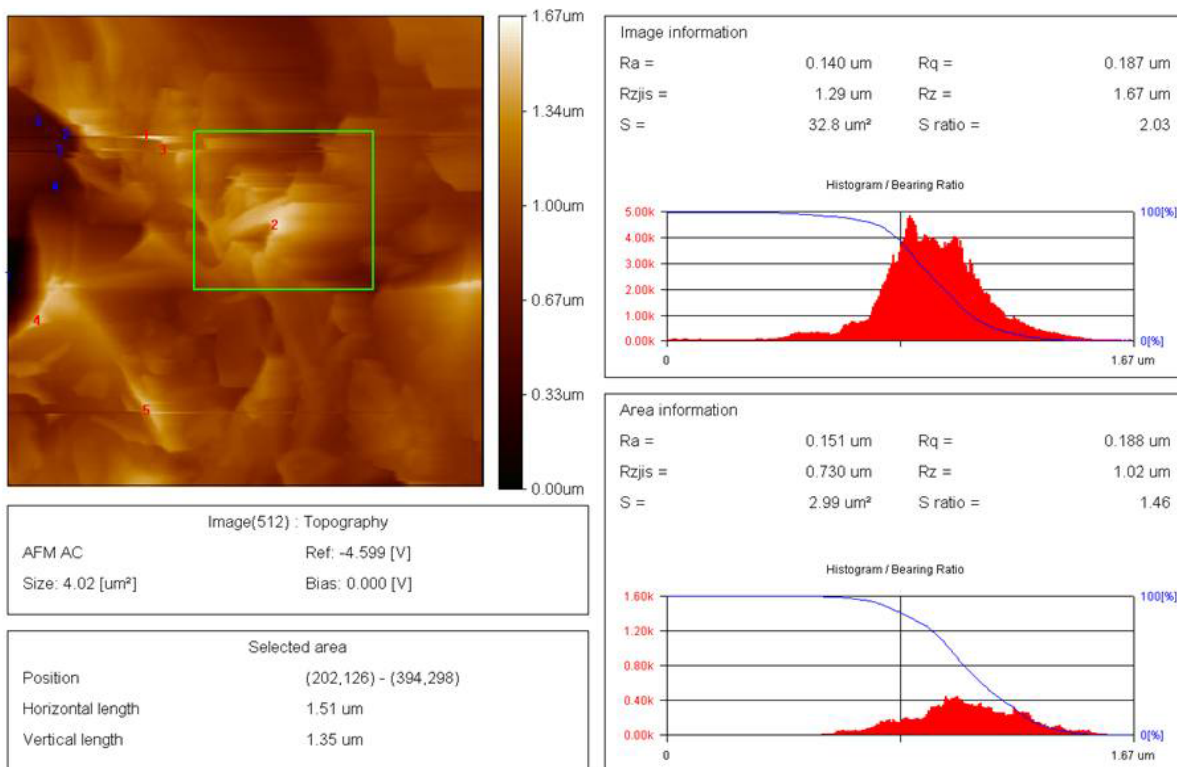
Figure SI-I. AFM images of N-24 electrode surface
