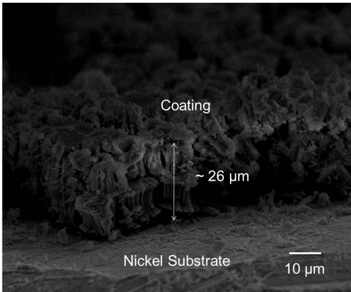
Figure SI-II. SEM image showing thickness of N-24 electrode.
