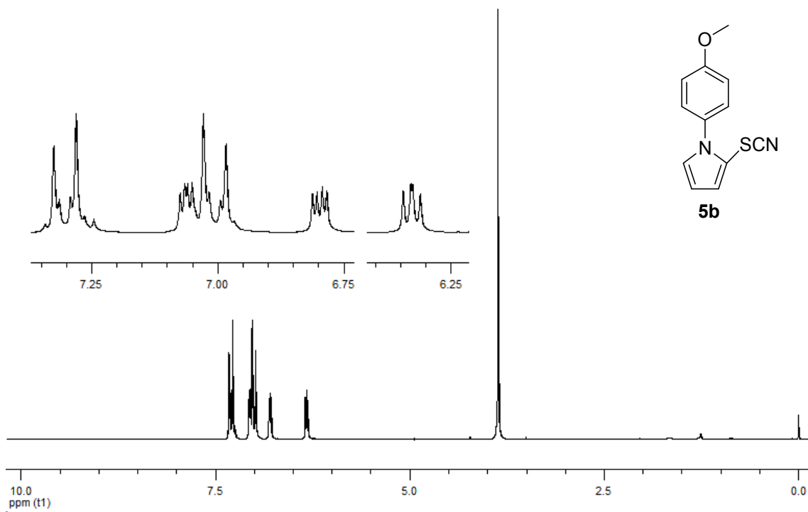
Figure S32. 200 MHz 1 H NMR spectrum of compound 5b in CDCl 3 .
