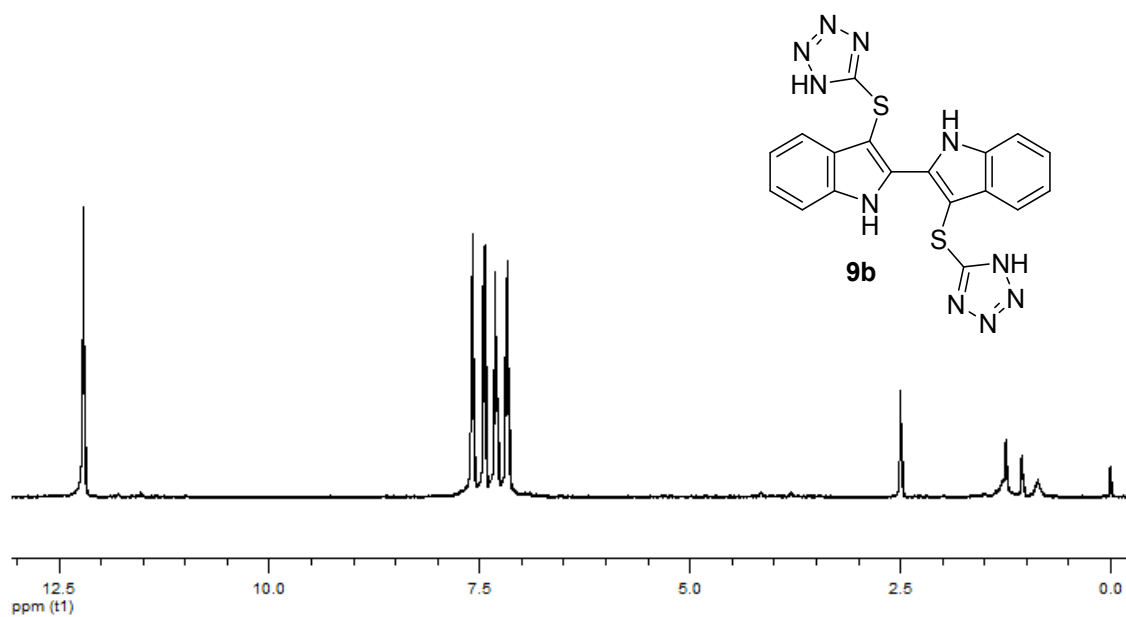
Figure S82. 400 MHz 1 H NMR spectrum of compound 9b in DMSO- d 6 .
