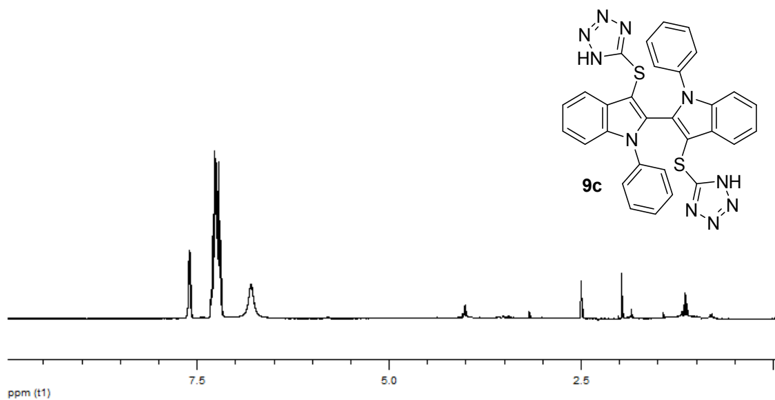
Figure S84. 400 MHz 1 H NMR spectrum of compound 9c in DMSO- d 6 .
