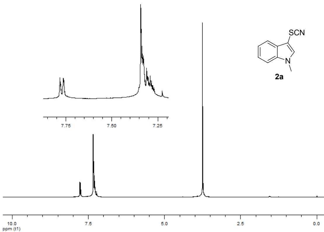
Figure S3. 400 MHz ^1\text{H} NMR spectrum of compound 2a in \text{CDCl}_3 .
