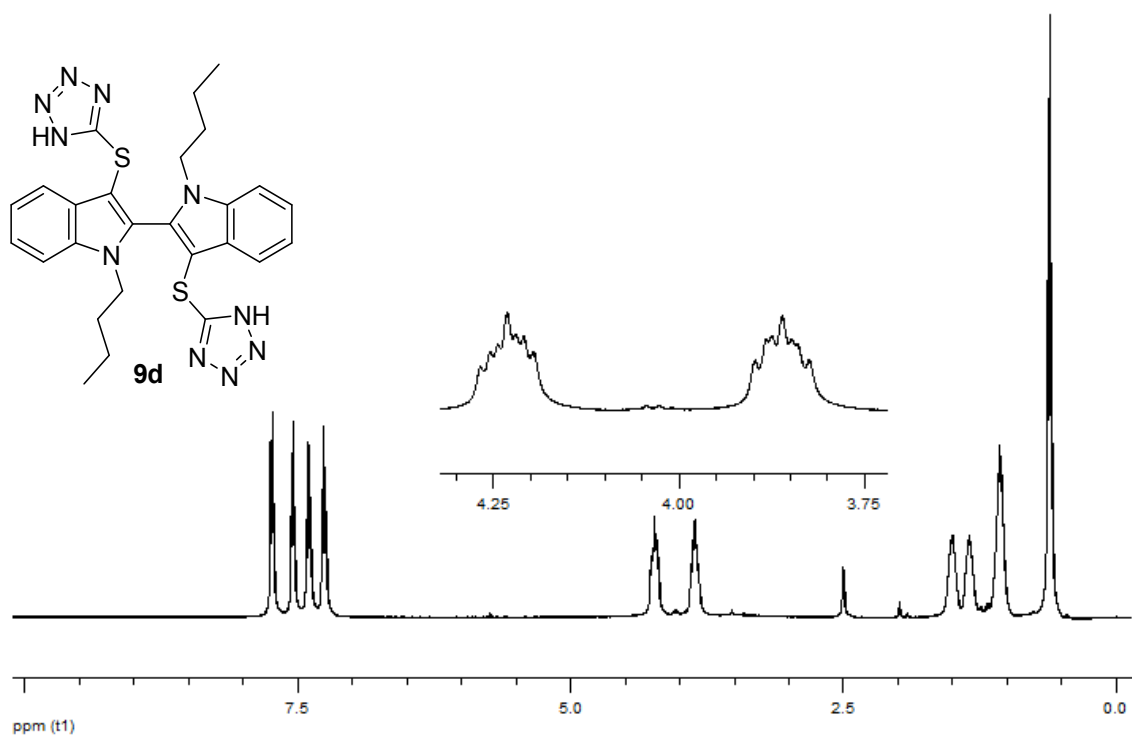
Figure S86. 400 MHz 1 H NMR spectrum of compound 9d in DMSO- d 6 .
