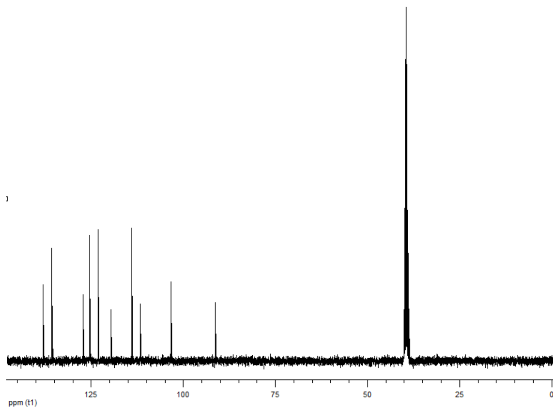
Figure S29. 100 MHz 13 C NMR spectrum of compound 2n in DMSO- d 6 .
