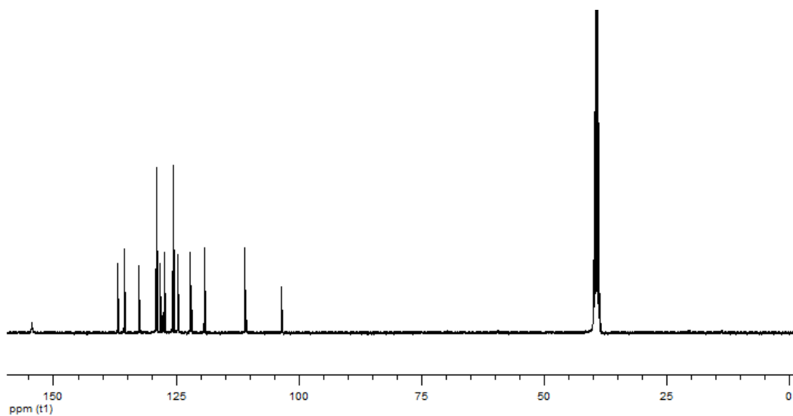
Figure S85. 100 MHz 13 C NMR spectrum of compound 9c in DMSO- d 6 .
