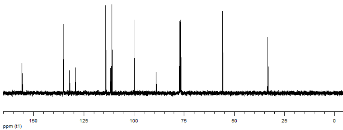
Figure S8. 100 MHz 13 C NMR spectrum of compound 2c in CDCl 3 .
