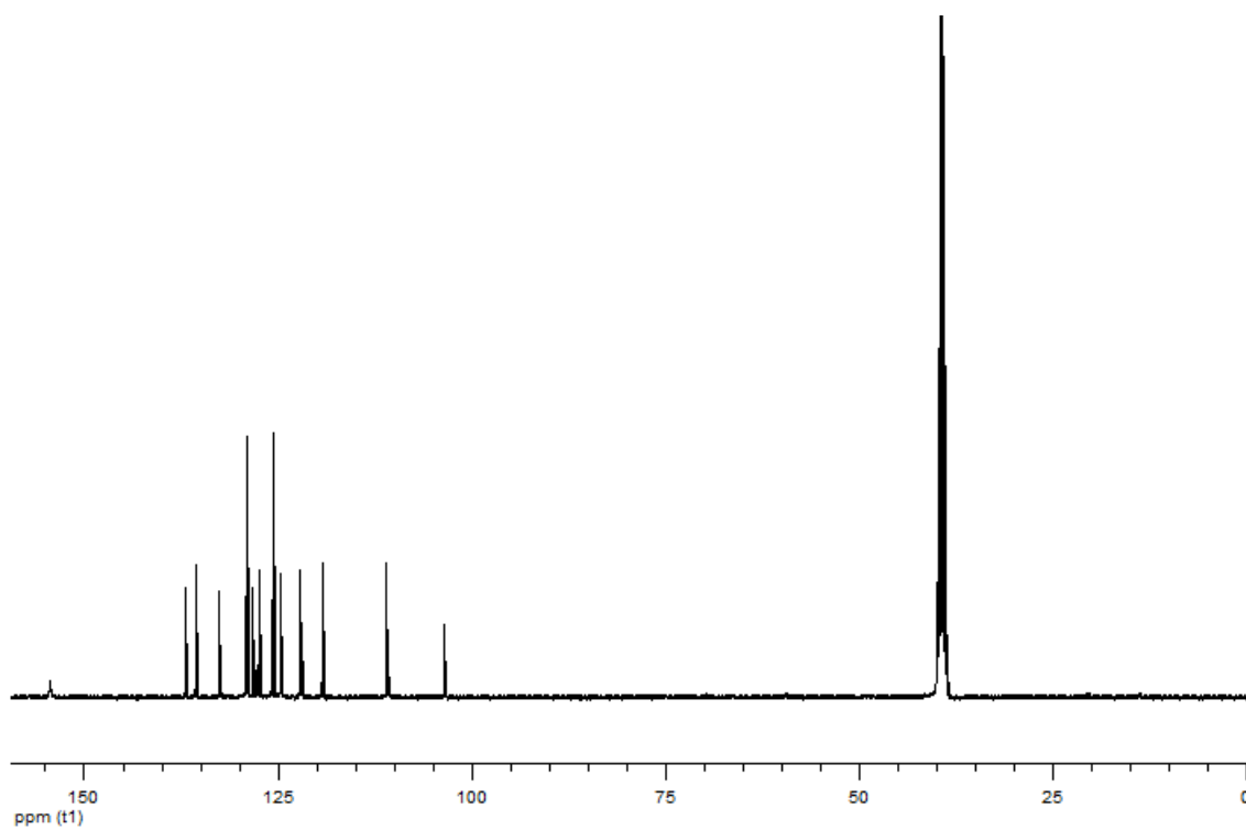
Figure S83. 100 MHz 13 C NMR spectrum of compound 9b in DMSO- d 6 .
