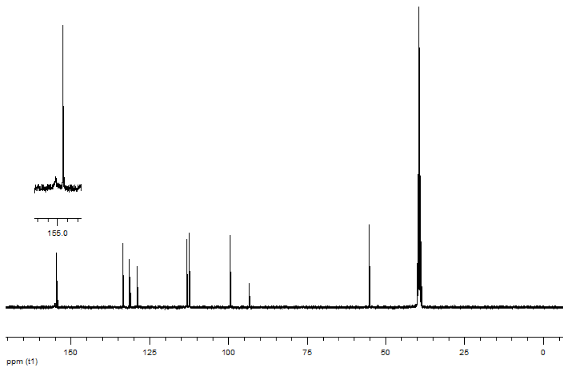
Figure S57. 100 MHz 13 C NMR spectrum of compound 3k in DMSO- d 6 .
