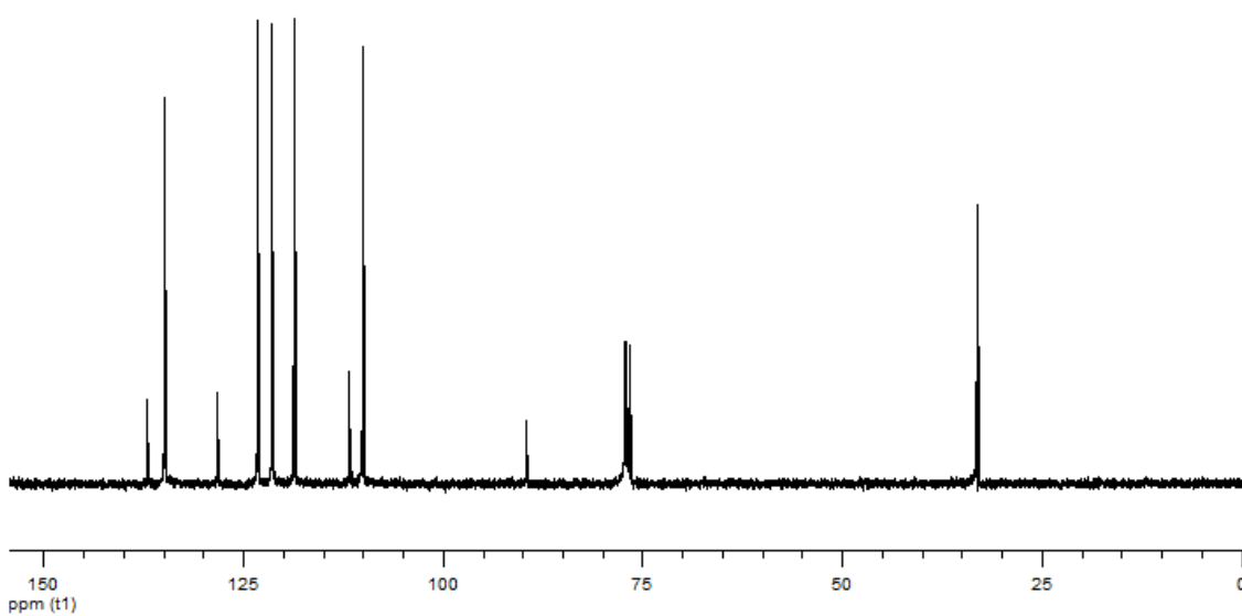
Figure S4. 100 MHz ^{13}\text{C} NMR spectrum of compound 2a in \text{CDCl}_3 .
