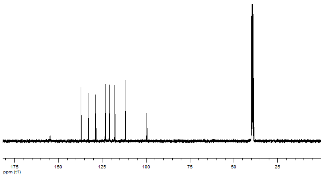
Figure S89. 100 MHz ^{13}\text{C} NMR spectrum of compound 9e in \text{DMSO-}d_6 .
