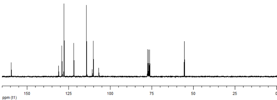
Figure S33. 50 MHz 13 C NMR spectrum of compound 5b in CDCl 3 .
