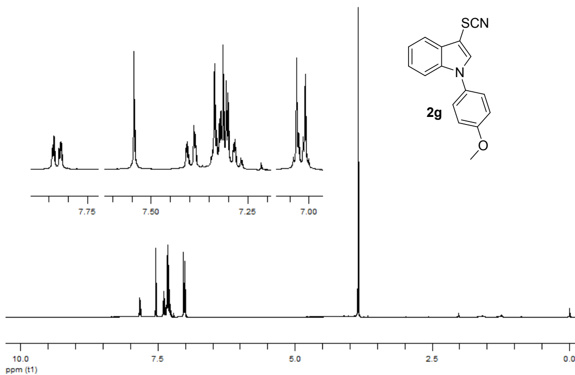
Figure S15. 400 MHz ^1\text{H} NMR spectrum of compound 2g in \text{CDCl}_3
