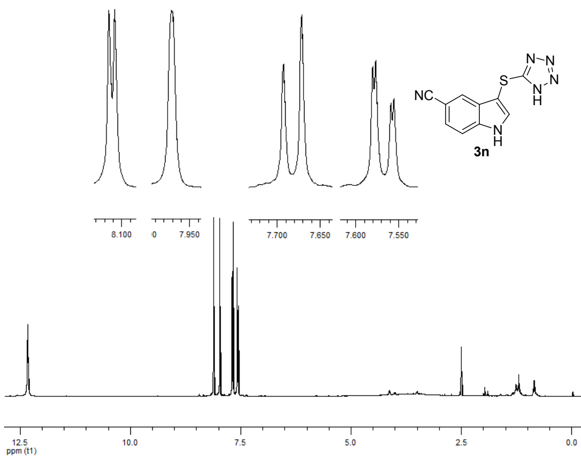
Figure S62. 400 MHz 1 H NMR spectrum of compound 3n in DMSO- d 6 .
