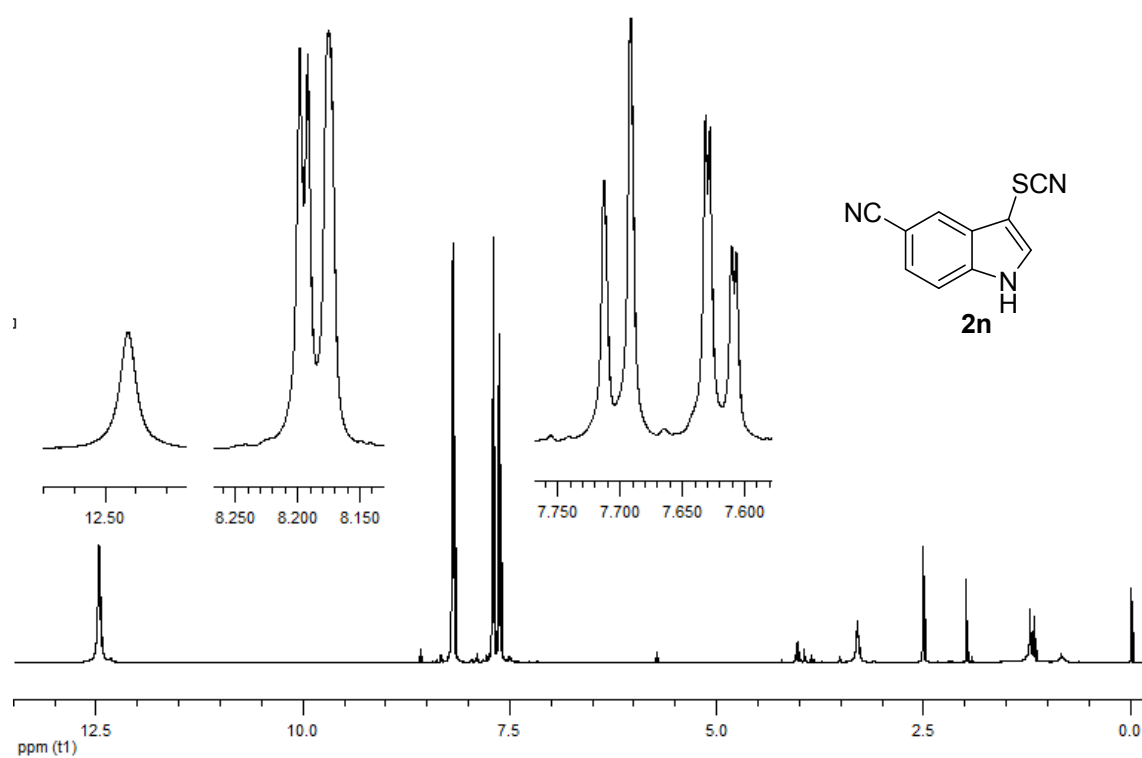
Figure S28. 400 MHz 1 H NMR spectrum of compound 2n in DMSO- d 6 .
