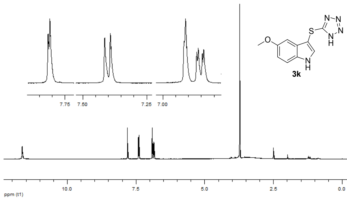
Figure S56. 400 MHz 1 H NMR spectrum of compound 3k in DMSO- d 6 .
