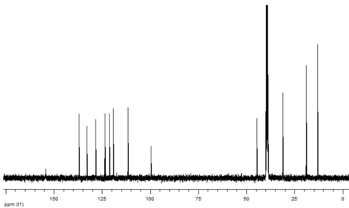
Figure S87. 100 MHz 13 C NMR spectrum of compound 9d in DMSO- d 6 .
