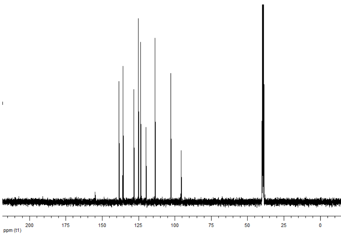
Figure S63. 100 MHz 13 C NMR spectrum of compound 3n in DMSO- d 6 .
