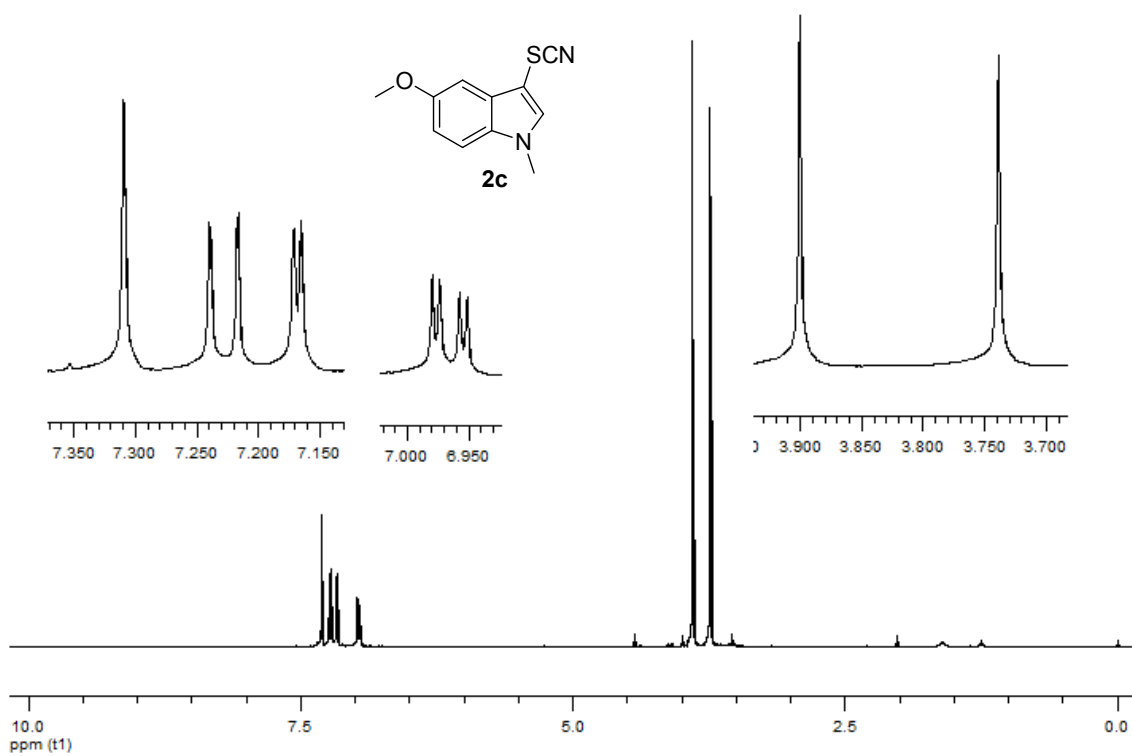
Figure S7. 400 MHz 1 H NMR spectrum of compound 2c in CDCl 3 .
