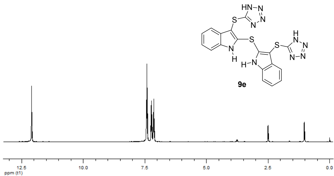
Figure S88. 400 MHz ^1\text{H} NMR spectrum of compound 9e in \text{DMSO-}d_6 .
