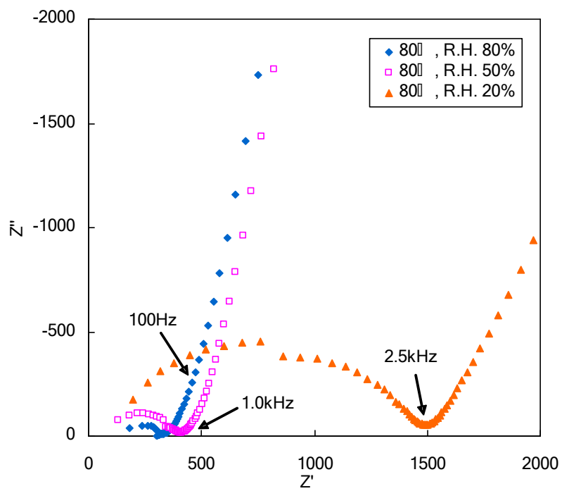
Figure S2 Cole-cole plots of delaminated LDH at 80°C under different relative humidity
