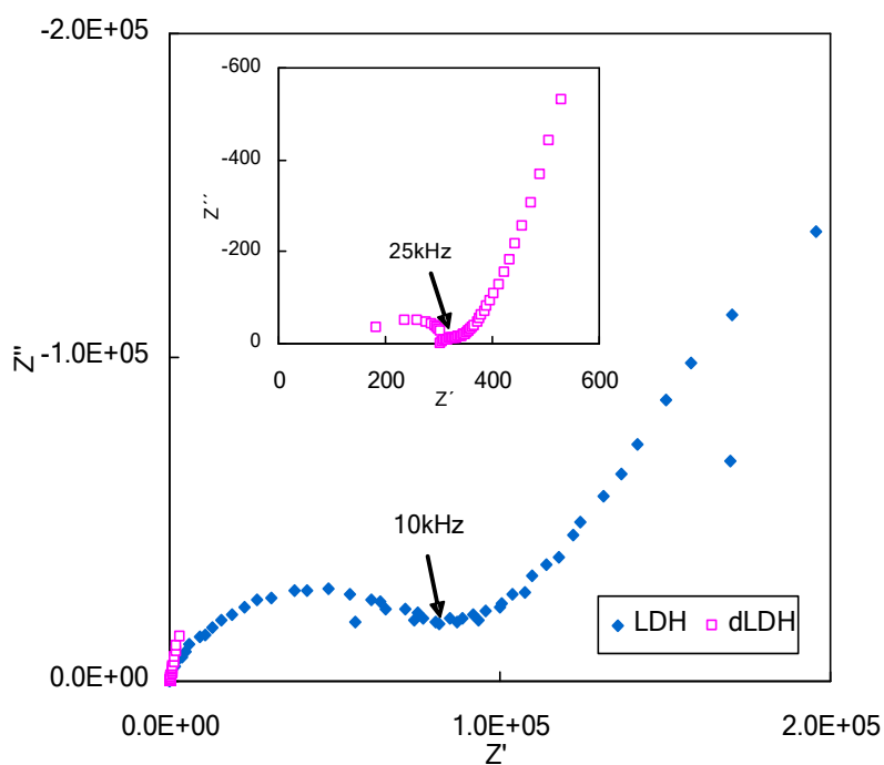
Figure S1 Cole-cole plots of as prepared LDH and delaminated LDH at 80°C R.H. 80%
