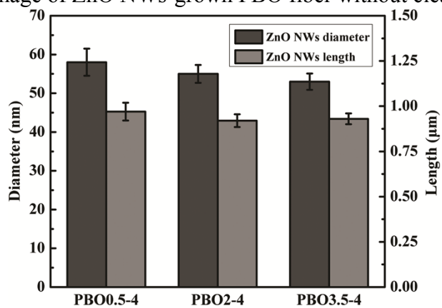
Figure S2. Effect of [S]/[G] ratio on the dimension of ZnO NWs.
