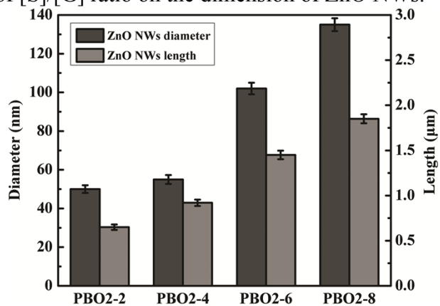
Figure S3. Effect of growth time on the dimension of ZnO NWs.
