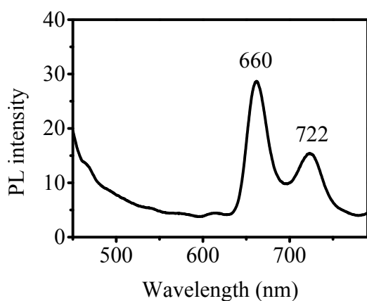
Fig. S2. Fluorescence spectrum of the TAPPI in solid state. \lambda_{\text{ex}} = 408 nm.
