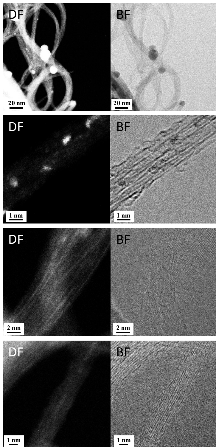
Figure S2. High-angle annular dark field and bright field images of Mo-encapsulated single walled carbon nanotubes.
