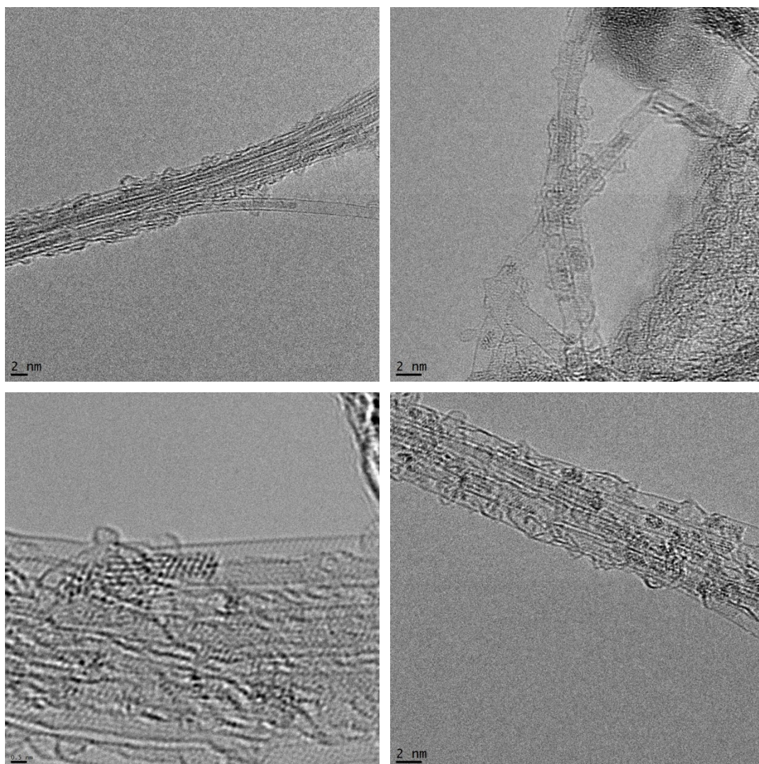
Figure S1. High resolution transmission electron microscopic images of Mo-encapsulated single walled carbon nanotubes.
