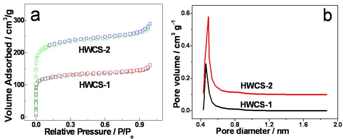
Figure S1(a) N 2 adsorption-desorption isotherms and (b) pore size distributions on HWCS-1 and HWCS-2.
