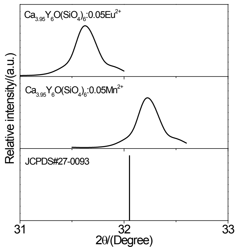
Fig.S1. Enlarged diffraction peak at 2\theta=31\text{-}33^\circ .
