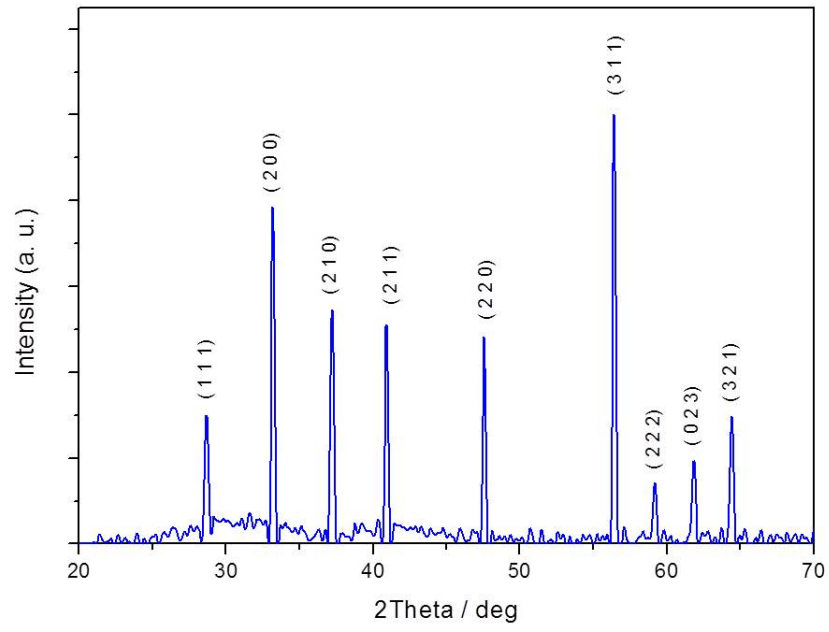
Figure S3: XRD pattern of the grinded commercial iron pyrite mineral.
