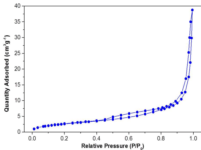
Figure S1: Nitrogen adsorption/desorption isotherm for the as-synthesized pyrite FeS 2 after solvothermal reaction at 180 °C for 18 h.
