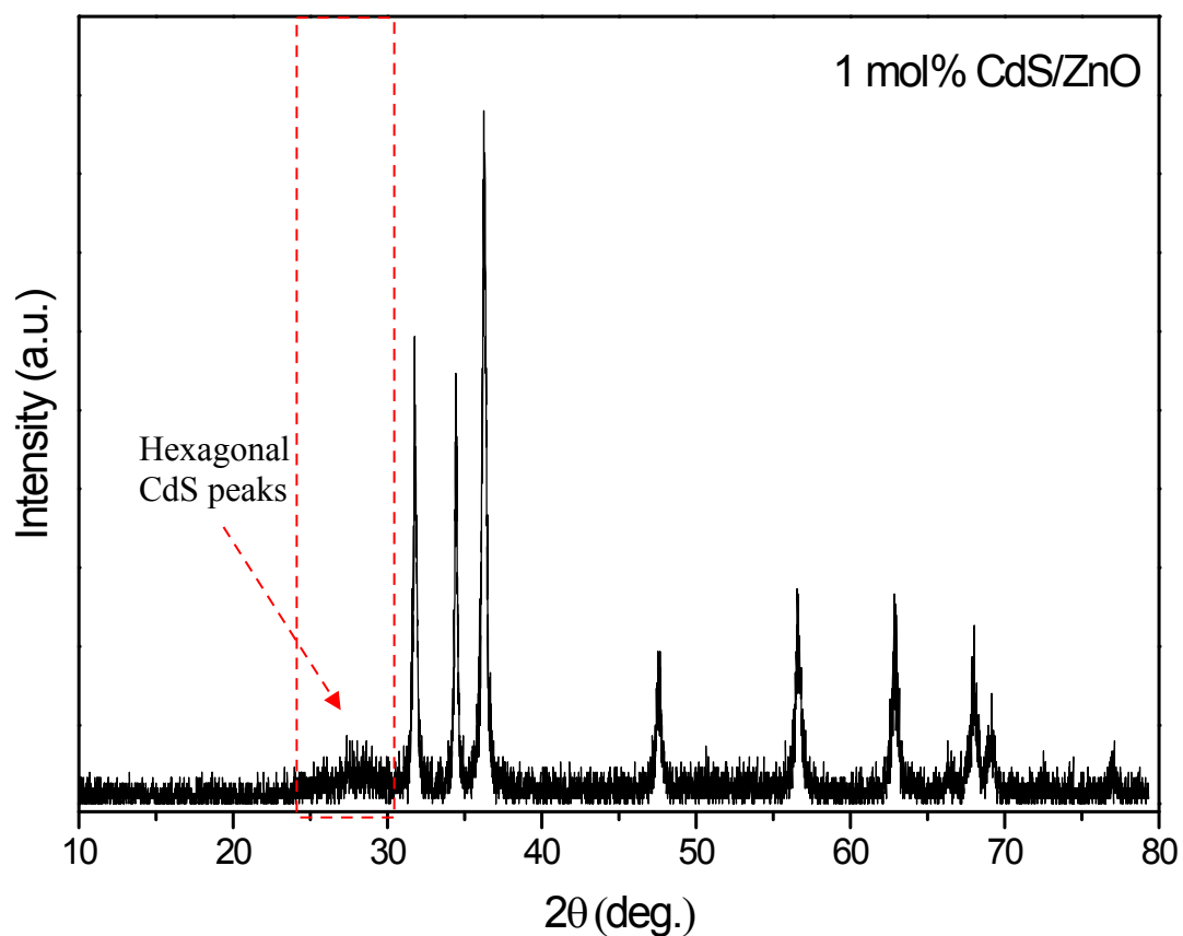
Figure S1. XRD of 1 mol% CdS/ZnO nanocomposite
