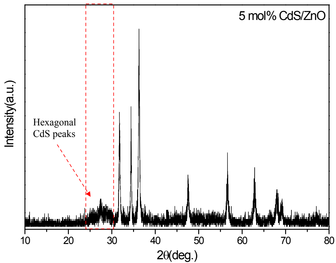
Figure S2. XRD of 5 mol% CdS/ZnO nanocomposite
