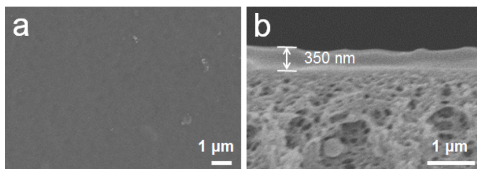
Fig. S1 (a) surface and (b) cross-sectional morphologies of a PECNFM2.1 membrane after 18 h continuous NF test.
