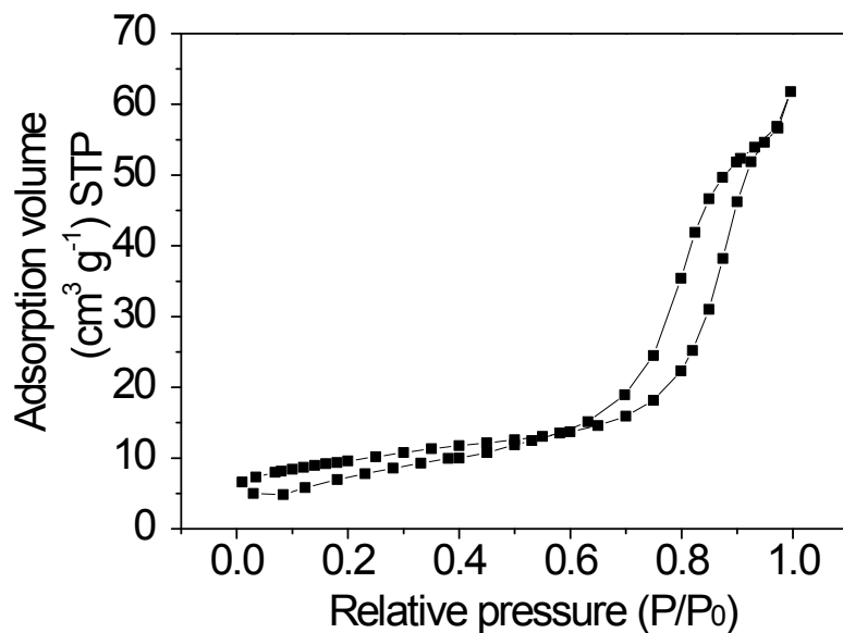
N 2 adsorption–desorption isotherms of synthesized WS-Mn 3 O 4
