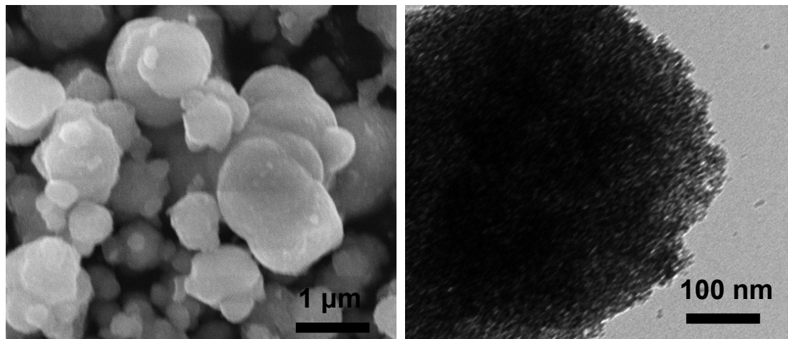
(a) SEM of WS- Mn 3 O 4 nanoparticles TEM (b) TEM images of WS-Mn 3 O 4 nanoparticles
