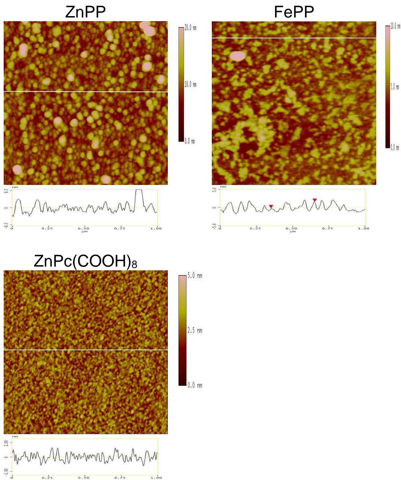
Figure 8 : AFM images ( 1 \times 1 \mu\text{m}^2 ) of macrocycle layers grafted without coupling reagent (CDI).
