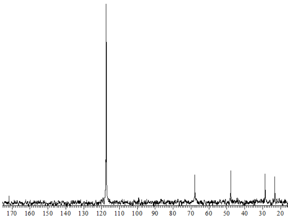
Figure S6. ^{13}\text{C} NMR spectrum ( \text{CD}_3\text{CN} ) of 2b .
