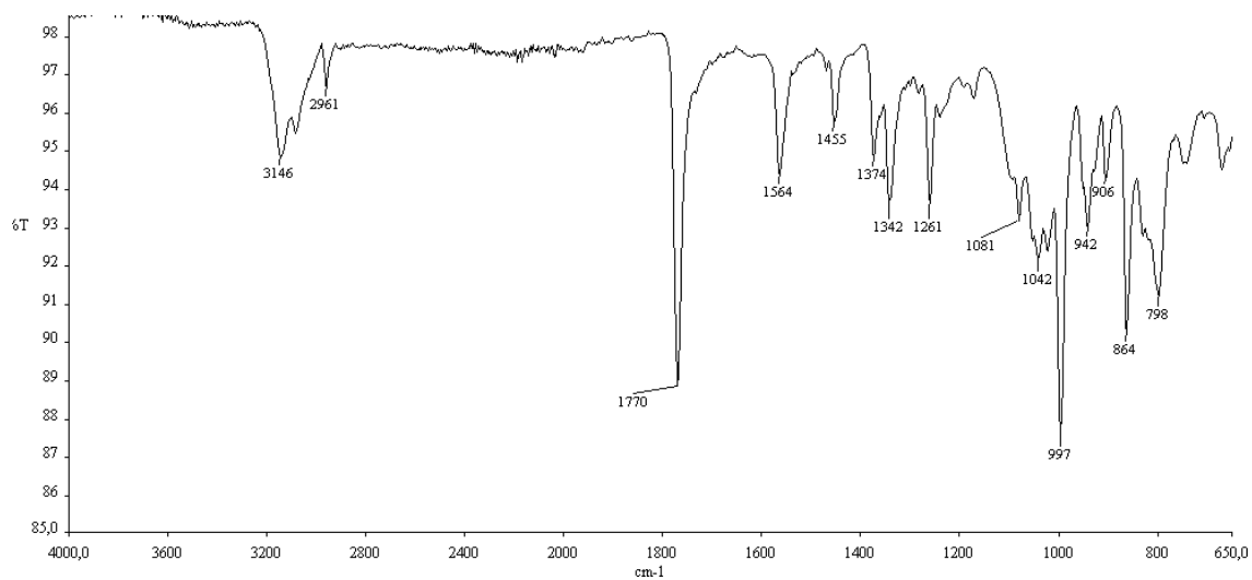
Figure S2. IR spectrum (solid state) of 2b .
