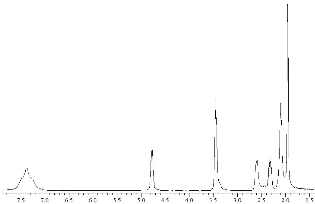
Figure S3. ^1\text{H} NMR spectrum ( \text{CD}_3\text{CN} ) of 2a .
