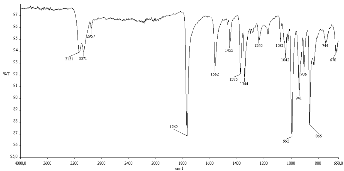
Figure S1. IR spectrum (solid state) of 2a .
