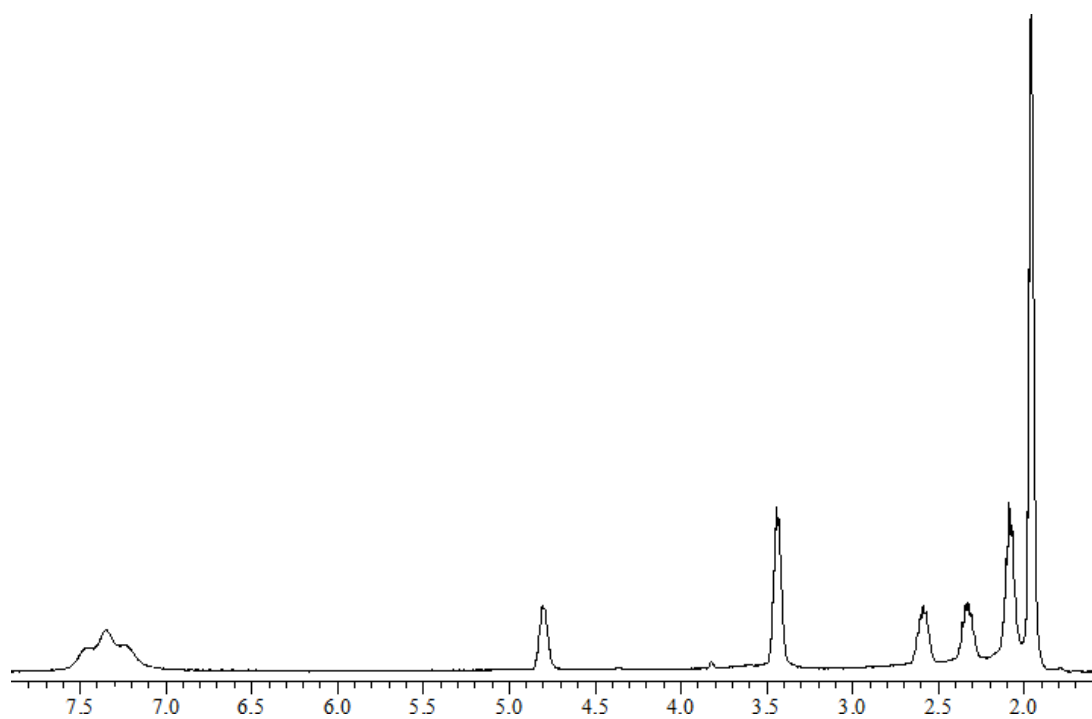
Figure S4. ^1\text{H} NMR spectrum ( \text{CD}_3\text{CN} ) of 2b .
