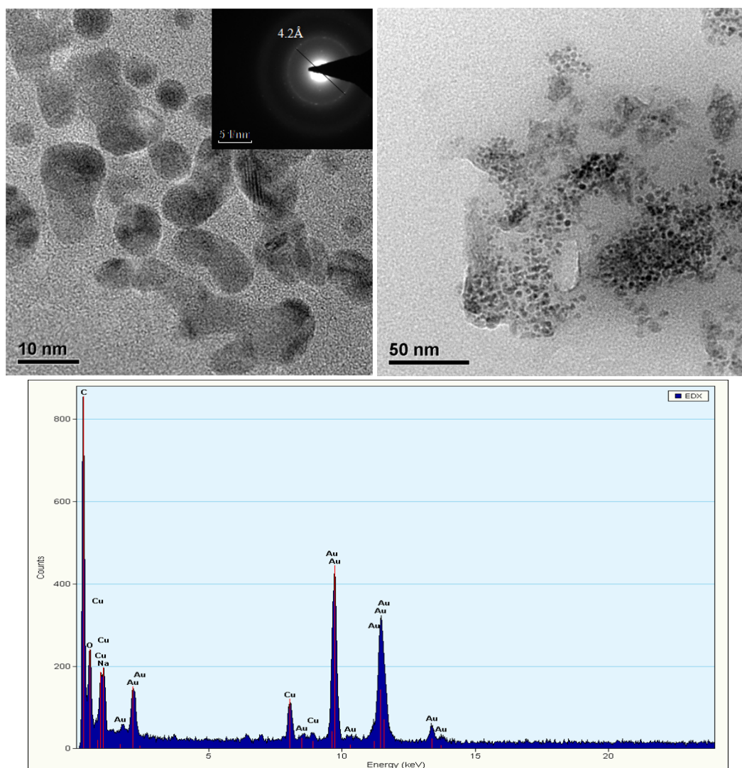
Fig. S1 HRTEM of Chitosan coated Cu 2 O in high magnification (top left) and low magnification (top right) with SAED pattern (top left; inset) and EDX pattern (bottom).
