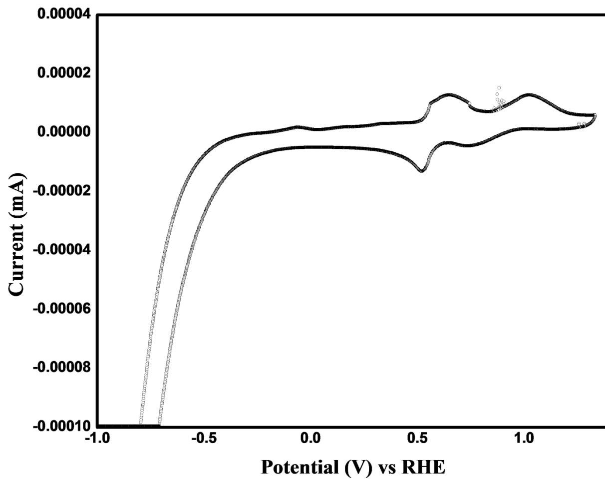
Fig. S2 CV for control \text{Cu}_x\text{O} at scan rate of 50 \text{ mVs}^{-1} .
