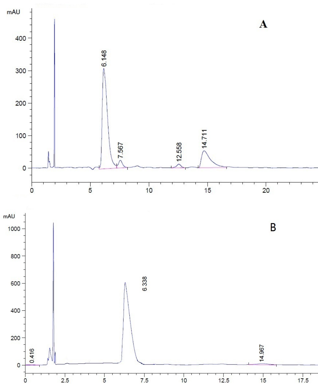
Fig.6 A. HPLC chromatogram of alkaloids of Dature metel L. B. HPLC chromatogram of atropin after separation by MWCNT-1 C. HPLC chromatogram of anisodamine after separation by MWCNT-1
