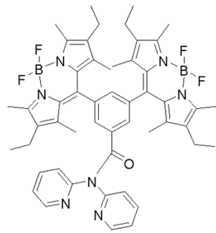
Bodipy-DPy
