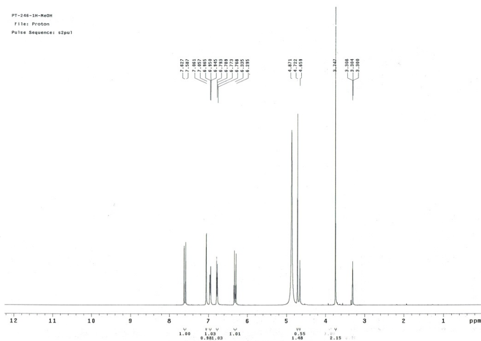
1) ^1\text{H} NMR spectrum of caffeoylglycolic acid methyl ester
