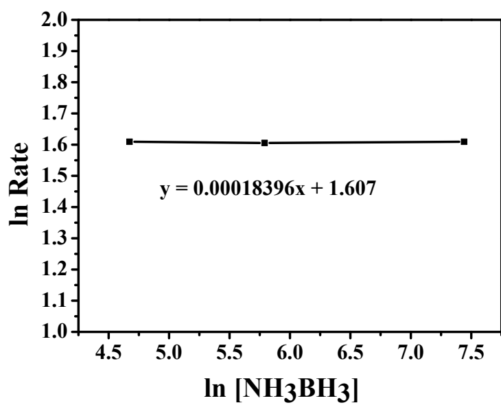
Fig. S2 The plot of hydrogen generation rate versus the concentration of AB.
