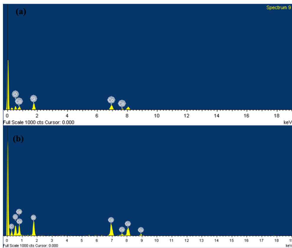
Fig. S1 EDX of (a) Co/SAG and (b) Co/MCM-41.
