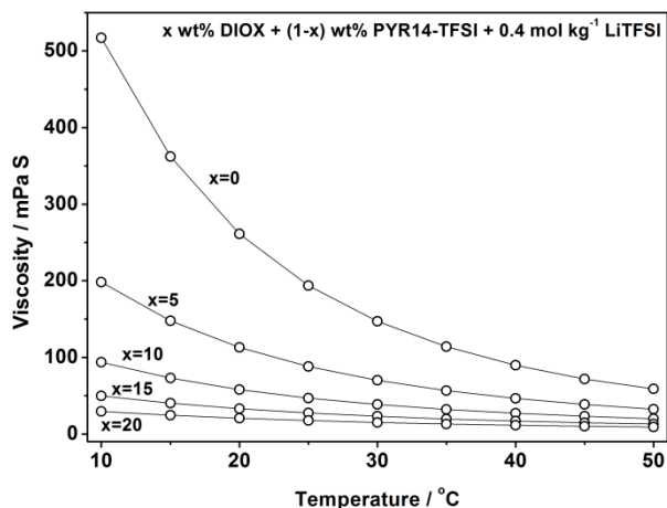
Figure S1 Viscosity as a function of temperature for the mixed electrolytes.
