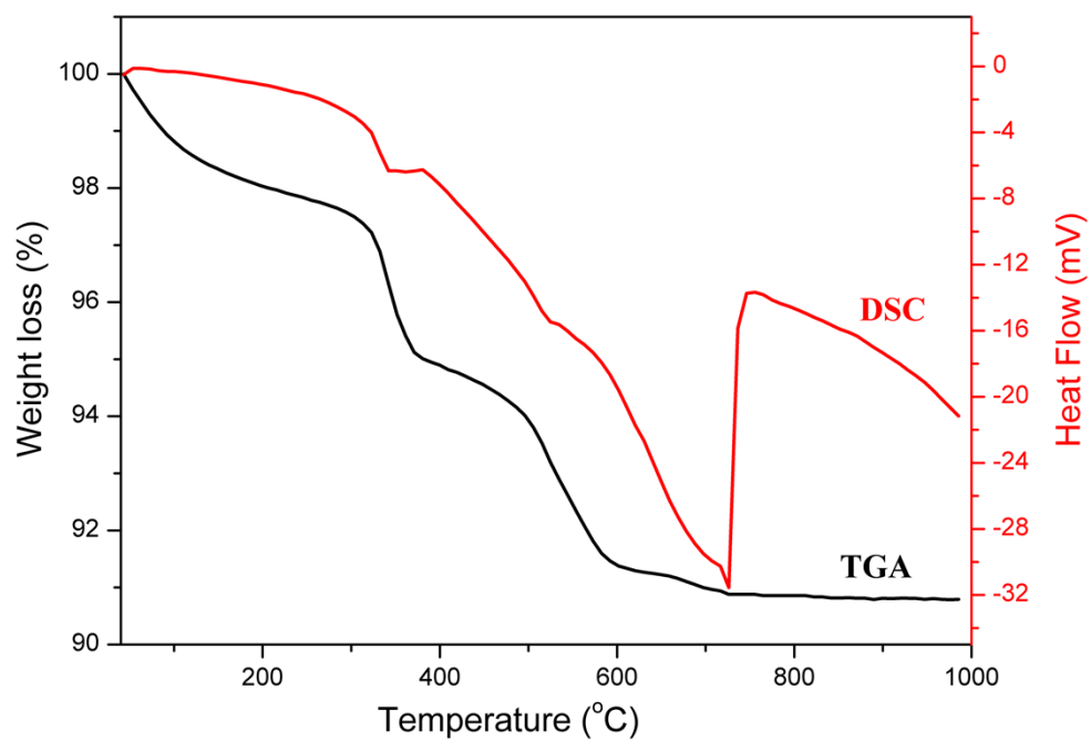
Fig. S1 TGA-DSC curves of the raw materials ( \text{Li}_2\text{CO}_3 , \text{La}_2\text{O}_3 and \text{WO}_3 ) after grinding.
