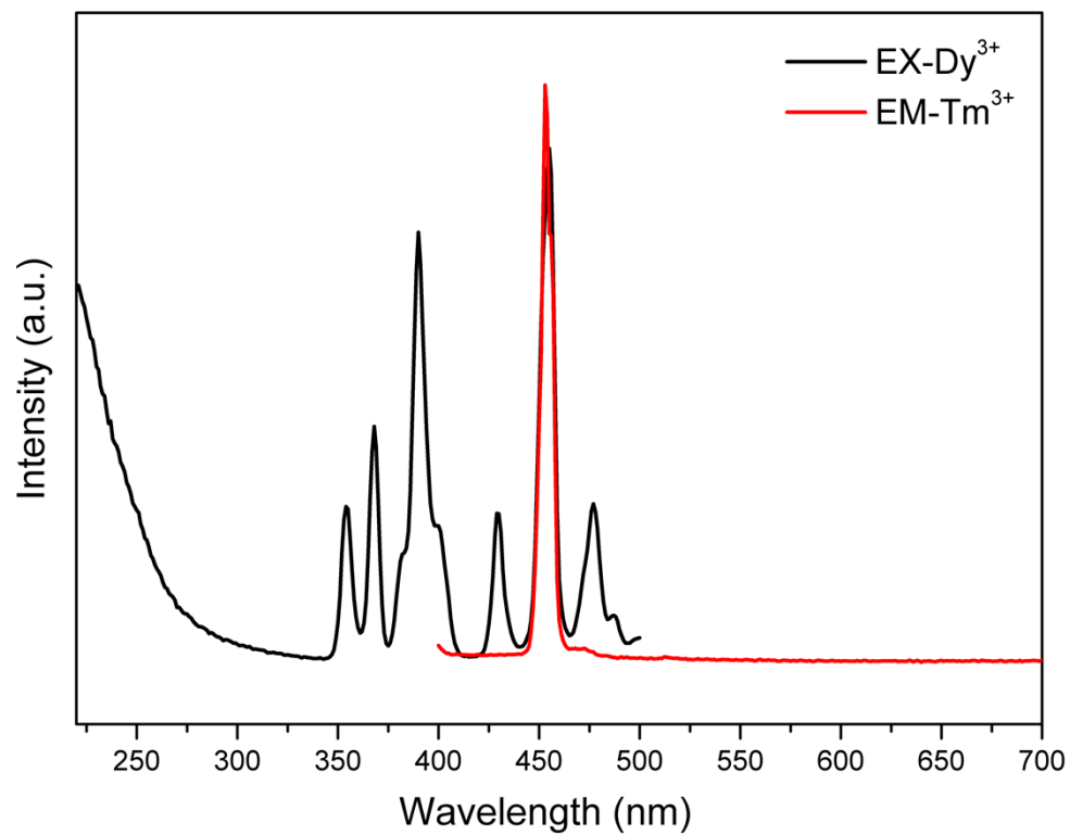
Fig. S2 Spectral overlap between the excitation spectrum of \text{LiLa}(\text{WO}_4)_2:0.04\text{Dy}^{3+} and emission spectrum of \text{LiLa}(\text{WO}_4)_2:0.04\text{Tm}^{3+} .
