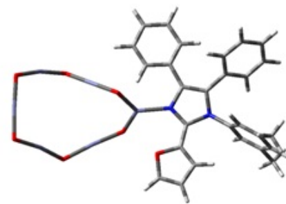
Imidazole-Zn 6 O 6
