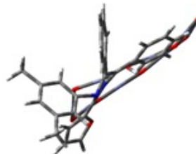
Imidazole-Zn 8 O 8
