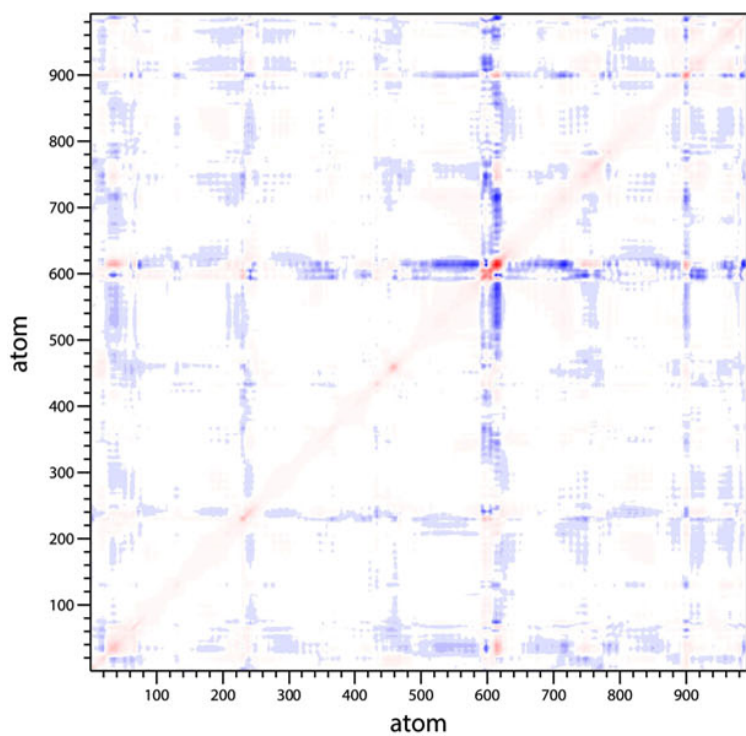
Covariance
