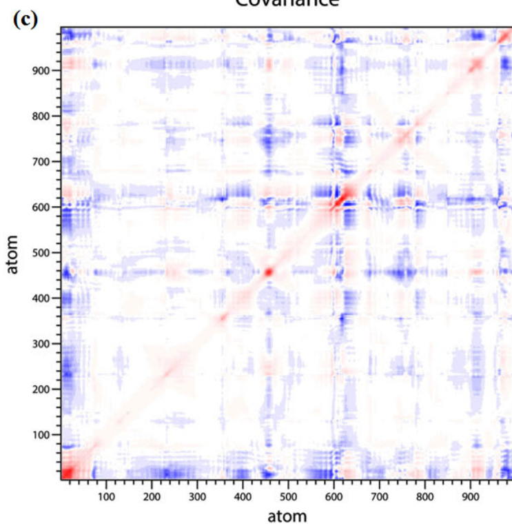
Covariance
