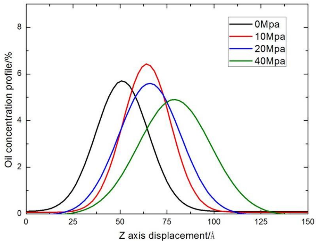
Figure s1. Oil concentration profile in final configuration of N 2 driving oil transport in shale channel with N 2 initial pressure of 0 Mpa, 10 Mpa, 20 Mpa and 40 Mpa.
