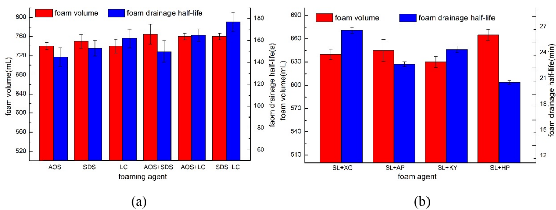
Fig. 1 Foam properties for various foam solutions. (a) Surfactant foam solutions of which total concentration was 0.15 wt%, (b) Polymer-surfactant foam solutions of which polymer concentration and surfactant concentration were both 0.15 wt%.
