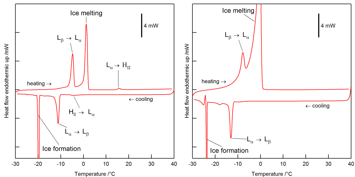
Figure 1. Differential scanning calorimetry (DSC) traces for DOPE fully hydrated in water and DOPE fully hydrated in a water/glucose solution with a lipid:glucose molar ratio 1:0.5. The lipid volume fraction of each sample is 0.5. DSC was performed on a Perkin-Elmer Pyris A DSC with intracooler. Temperature scan rate was 10 °/min.
