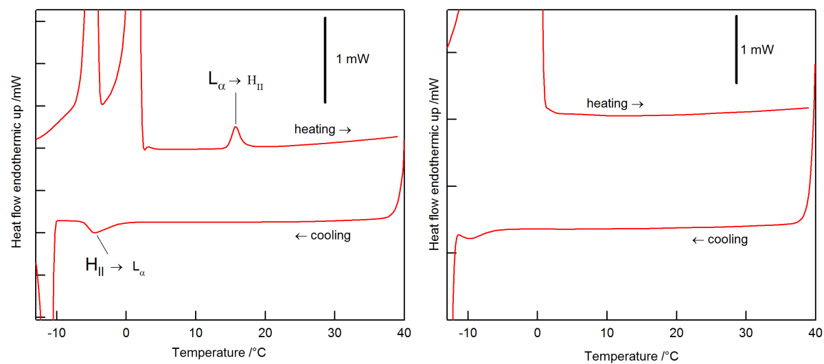
Figure 2. As above on an expanded vertical axis.
