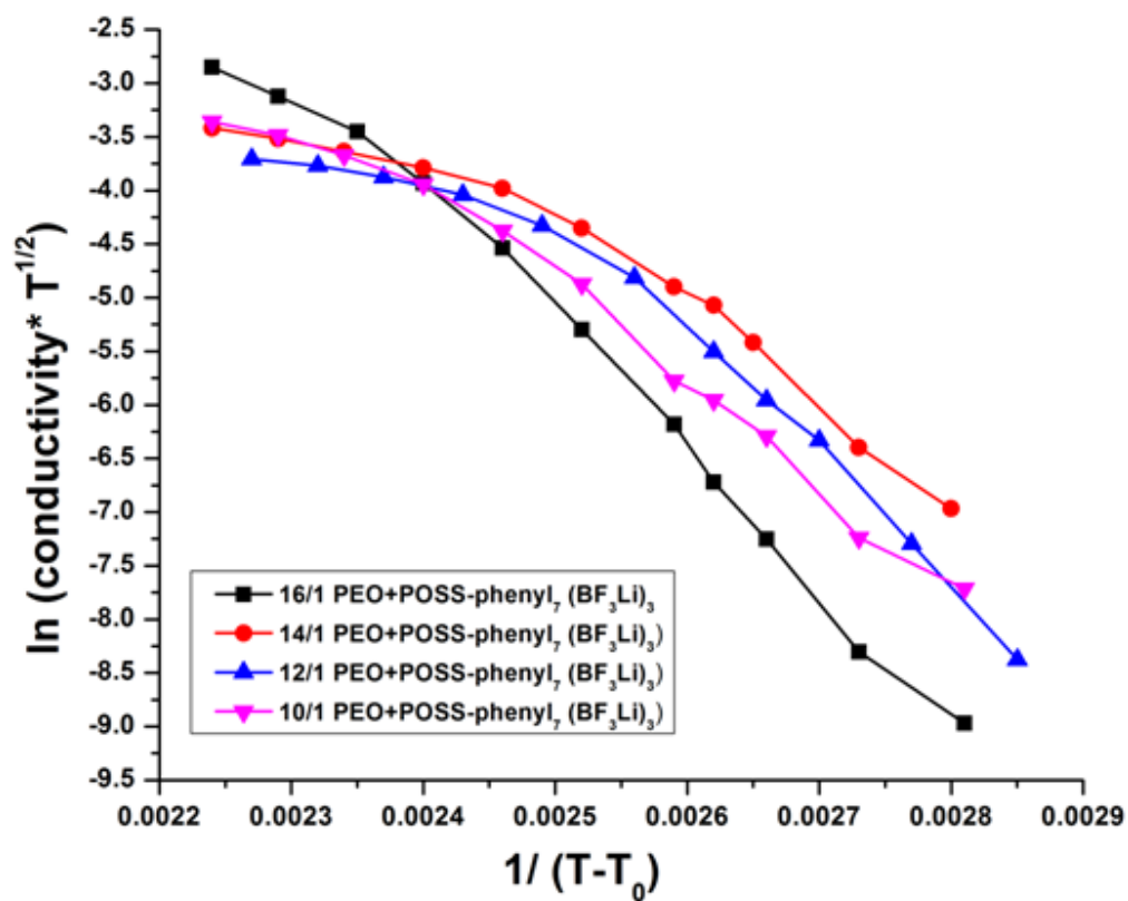
Figure 1. VTF plots of \text{POSS-phenyl}_7(\text{BF}_3\text{Li})_3/\text{PEO} as a function of O/Li ratio
