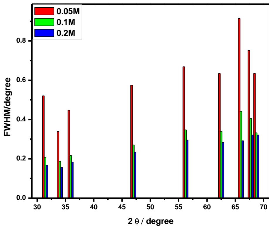
Figure S1. FWHM values of XRD diffraction peaks of ZnO nanoflowers synthesized at different precursor concentrations.
