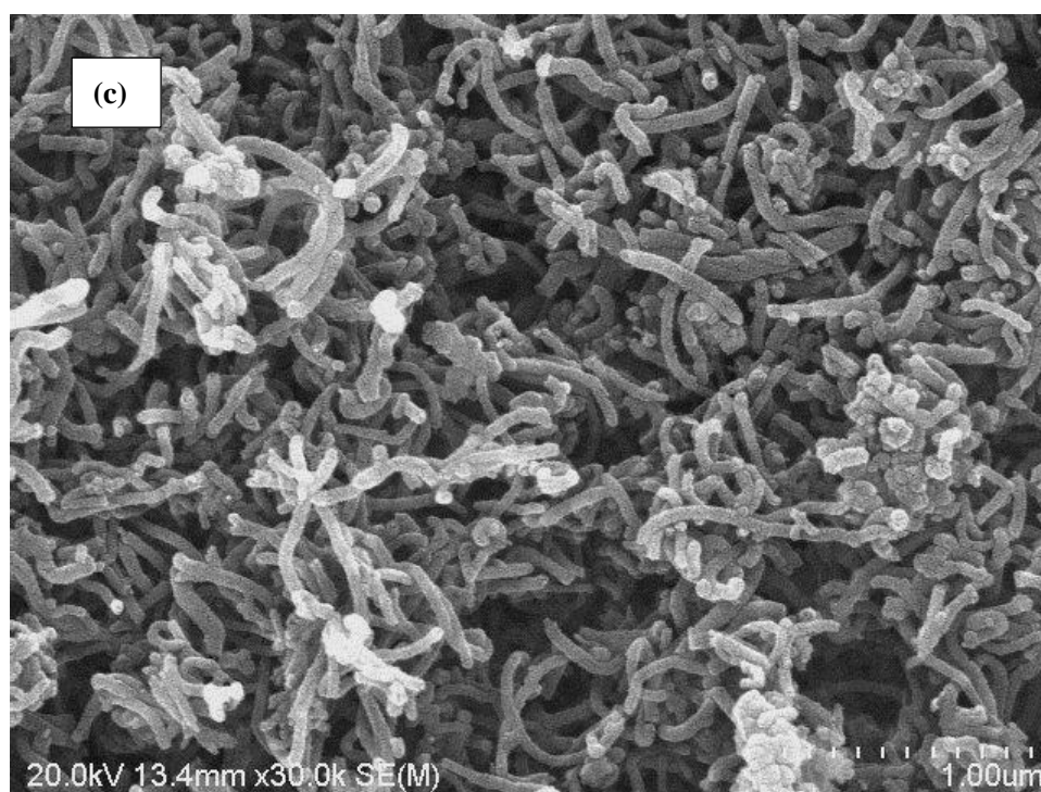
Fig.S1 SEM images of (a) CNTs, (b) CNTs@PPy and (c) NC-CNTs
