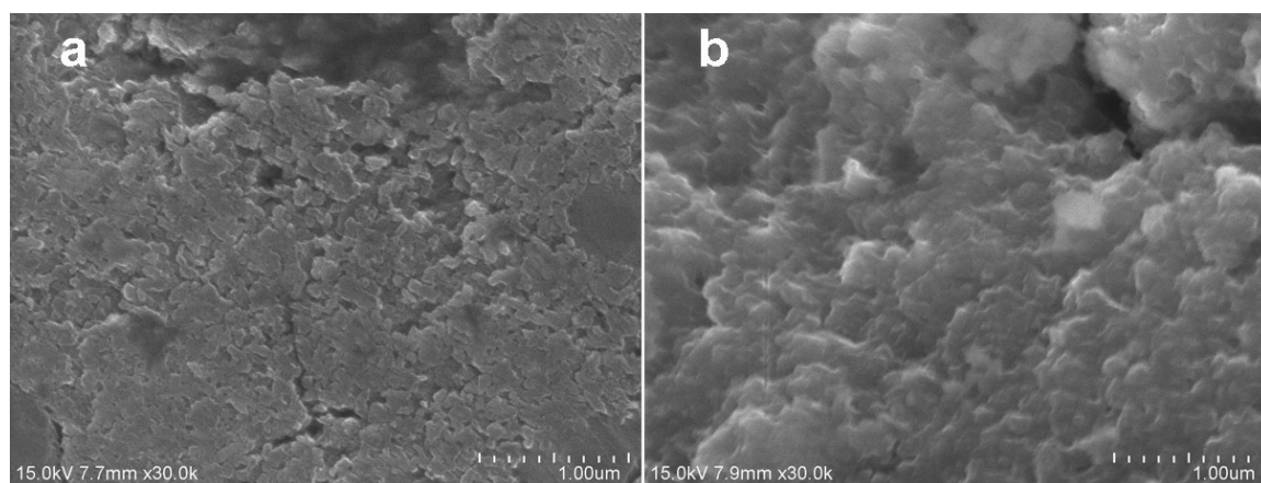
Figure S1 SEM images of \text{Fe}_3\text{O}_4/\text{C}@ CNT electrode sheets (a) before and (b) after 200-discharge/charge cycles. A cotton-like gel film is clearly seen in the cycled electrode.
