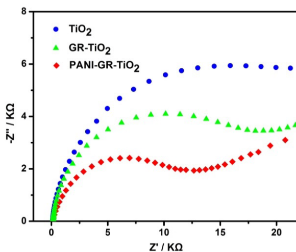
Fig. S2 EIS spectra of the TiO 2 , binary GR-TiO 2 , ternary PANI-GR-TiO 2 electrodes.
