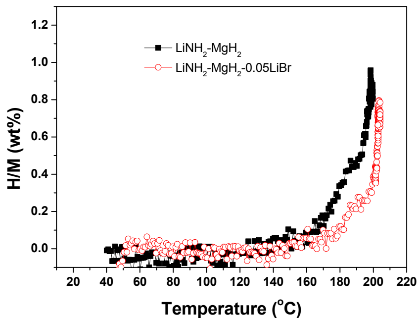
Fig. S1 Hydrogenation curves of the fully dehydrogenated LiNH 2 -MgH 2 and LiNH 2 -MgH 2 -0.05LiBr samples under 100 bar of H 2 pressure.
