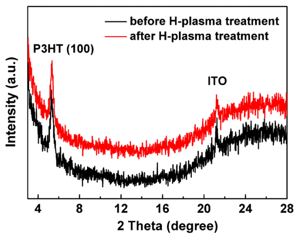
Fig. S1 XRD patterns of ITO/PEDOT:PSS/P3HT:PCBM/ZnO film measured before and after H-plasma treatment for 5 min.
