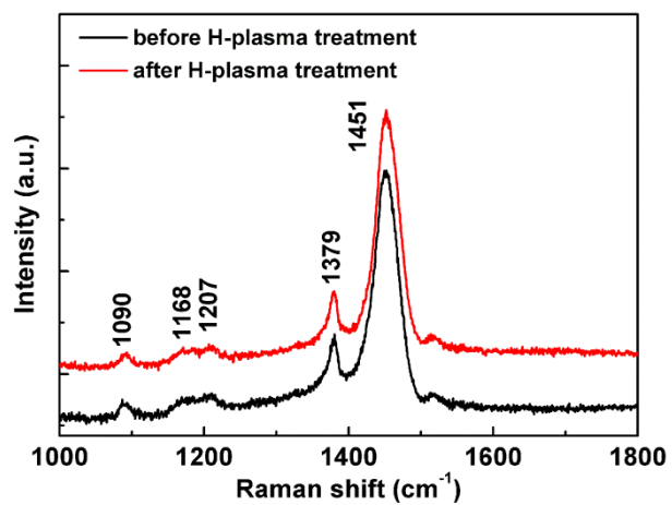
Fig. S2 Raman spectra of Si/P3HT:PCBM/ZnO film measured before and after H-plasma treatment for 5 min.
