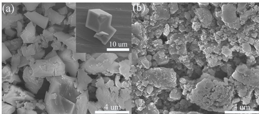
Fig. S2 The SEM images of CC-1 (a) and CC-2 (b) particles. The upper right image was the raw CC particle before grinding.
