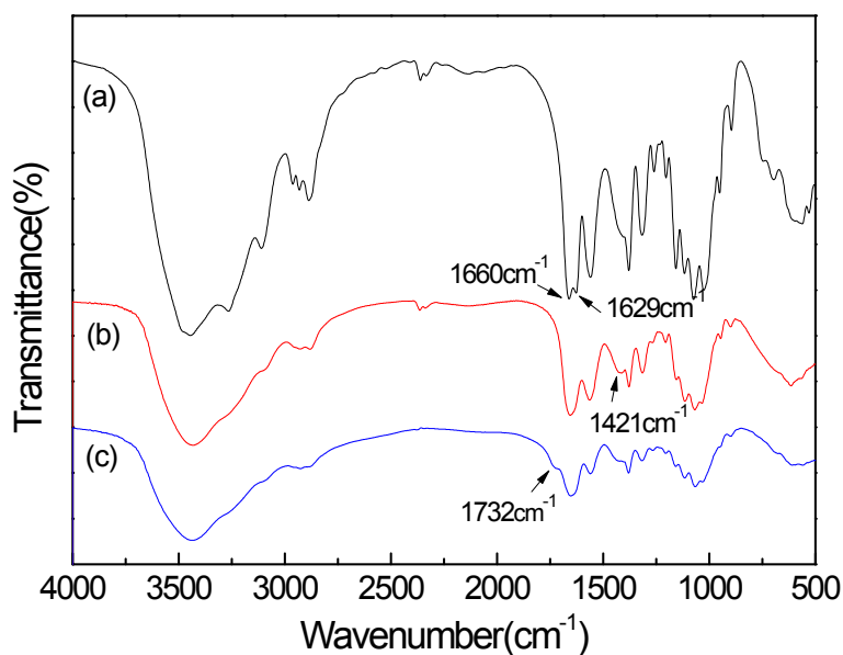
Fig. S1 FT-IR spectra of original chitin(a), acrylamide-modified chitin(AMC3) (b) and acrylamide-modified chitin hydrogel(AMCH3) (c).
