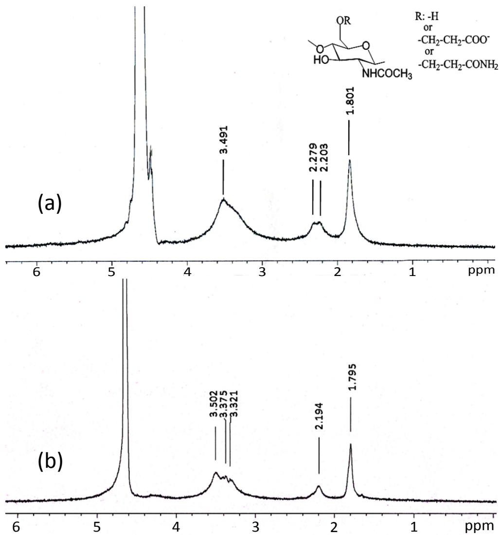
Fig. S2 1 H-NMR spectrum of acrylamide-modified chitin (a) and hydrolyzed acrylamide-modified chitin (b).
