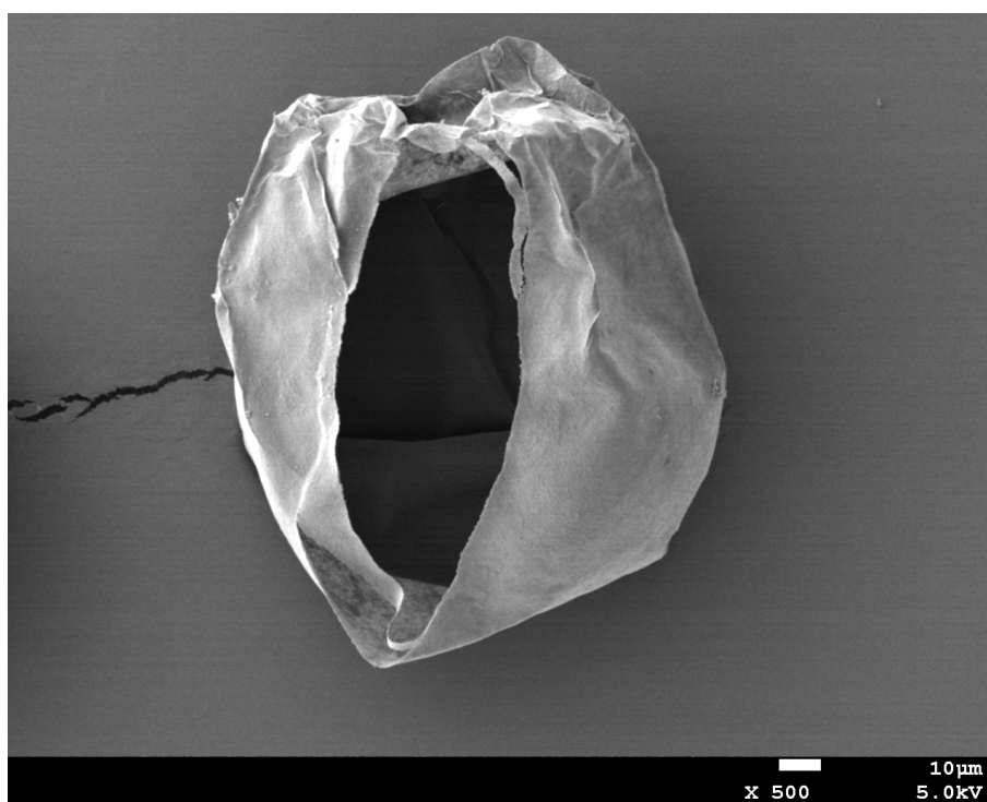
Fig. S1. SEM image of a ruptured APSi microcapsule after re-soaking in \text{CaCl}_2 solution. Scale bar is 10 \mu\text{m} .
