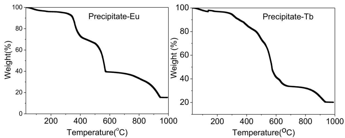
Figure S2. TGA curves of the complexes
