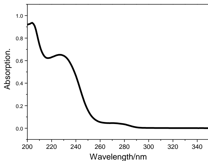
Figure S1. absorption spectrum of IL-ACC in EtOH ( 1.2 \times 10^{-5} \text{ M} )
