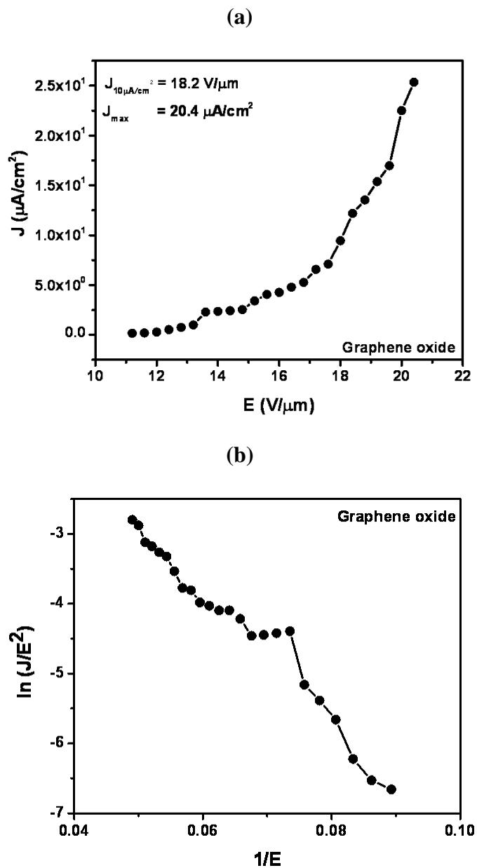
Figure S1 (a) Field emission current density ( J ) versus applied electric field ( E ), and (b) the corresponding F-N plot, of GO sheets
